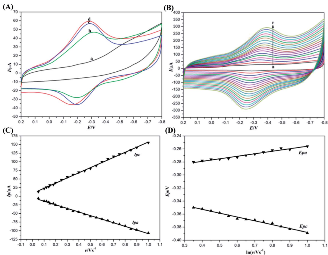
Fig. 4 (A) Cyclic voltammograms of (a) Nafion/ACA-GR/CILE, (b) Nafion/Mb-GR/CILE and (c) Nafion/Mb-ACA/CILE and (d) Nafion/Mb-ACA-GR/CILE in pH 7.0 PBS with the scan rate as 100 mV s -1 . (B) Cyclic voltammograms of Nafion/Mb-ACA-GR/CILE in pH 7.0 PBS at different scan rates (from a to r: 150, 200, 250, 300, 350, 400, 450, 500, 550, 600, 650, 700, 750, 800, 850, 900, 950, 1000 mV s -1 , respectively). (C) Linear relationship of the cathodic and anodic peak current ( I_p ) versus scan rate ( v ). (D) Linear relationship of the anodic and cathodic peak potential ( E_p ) versus \ln v .
