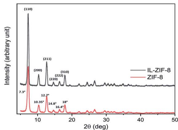
Fig. 1 PXRD patterns for the synthesized nanocomposite [BMIM]BF 4 @ZIF-8 (black line) and ZIF-8 (used as control compound) has been depicted in Fig. 1. The PXRD result depicts the presence of
