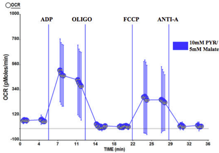
Figure 2. Highly Variable Pyruvate/Malate Assay. Highly variable 10 mM pyruvate/ 5 mM malate assay caused by incompletely mixing mitochondria from the mitochondrial stock in the substrate/MAS mix, thus leading to variable mitochondrial protein loading in each well. Mitochondrial protein loaded per well was 3.5 \mu g. Data represents n=3 paired biological replicates. OCR=Oxygen Consumption Rate; ADP= Adenosine diphosphate; Oligo= Oligomycin A; FCCP= Carbonyl cyanide-4-(trifluoromethoxy)phenylhydrazone; Anti-A= Antimycin A; PYR=Pyruvate. Please click here to view a larger version of this figure.
