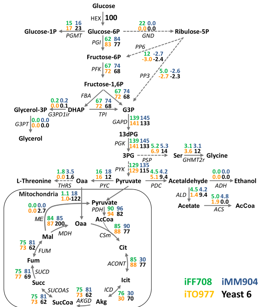
Fig. 2. Distribution of fluxes in the central metabolism predicted by pFBA for the models: iFF708 (green), iMM904 (blue), iTO977 (orange) and Yeast 6 (black). The flux values shown are normalized to a glucose uptake rate of 100 arbitrary units. Growth rates for each model: iFF708–0.11 h -1 , iMM904–0.11 h -1 , iTO977–0.11 h -1 , Yeast 6–0.09 h -1 . Reactions: ACNT- aconitase, ACS- acetyl-CoA synthetase, ADH- alcohol dehydrogenase, AKGD- alpha-ketoglutarate dehydrogenase, ALD- aldehyde dehydrogenase, CSm- citrate synthase, FBA- fructose 1,6-bisphosphate aldolase, FUM- fumarase, G3PD1ir- glycerol-3-phosphate dehydrogenase, G3PT- glycerol-1-phosphatase, GAPD- glyceraldehyde-3-phosphate dehydrogenase, GHMT2r- serine hydroxymethyltransferase, GND- 6-phosphogluconate dehydrogenase, HEX- hexokinase, ICD- mitochondrial isocitrate dehydrogenase, MDH- mitochondrial malate dehydrogenase, ME- mitochondrial malic enzyme, PDH- pyruvate dehydrogenase, PFK- phosphofruktokinase, PGI- phosphoglucose isomerase, PGK- 3-phosphoglycerate kinase, PGMT- phosphoglucomutase, PP3- sum of the non-oxidative reactions of the pentose phosphate pathway producing glyceraldehyde-3-phosphate, PP6- sum of the non-oxidative reactions of the pentose phosphate pathway producing fructose-6-phosphate, PSP- phosphoserine phosphatase, PYC- pyruvate carboxylase, PYK- pyruvate kinase, SUCD- succinate dehydrogenase, SUCOAS- succinyl-CoA ligase, THRS- threonine synthase, TPI- triose phosphate isomerase. Metabolites: 13dPG- 1,3-diphosphoglycerate, 3PG- 3-phosphoglycerate, AcCoA- acetyl-CoA, Akg- 2-oxoglutarate, Cit- citrate, DHAP- dihydroxyacetone-phosphate, Fum- fumarate, G3P- glyceraldehyde-3-phosphate, Icit- isocitrate, Mal - L-malate, Oaa- oxaloacetate, Ser- L-serine, Succ- succinate, SucCoa- succinyl-CoA. (For interpretation of the references to color in this figure legend, the reader is referred to the web version of this article.)
