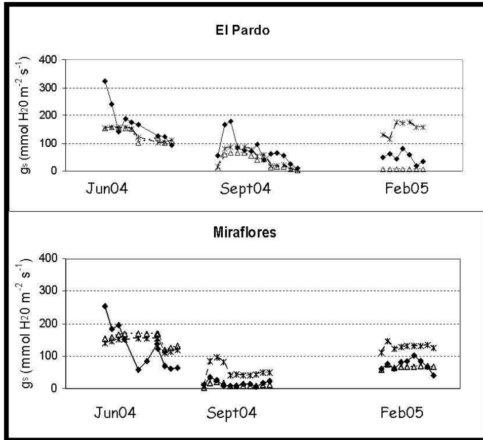
FIGURE 1. Calibration of the g_s model for Q. ilex using measured data at El Pardo and Miraflores during the period June 2004 to February 2005. ♦, measured data; *, calculated data based on literature review parameterization; Δ calculated data based on literature review parameterization including f_{SMD} function.
