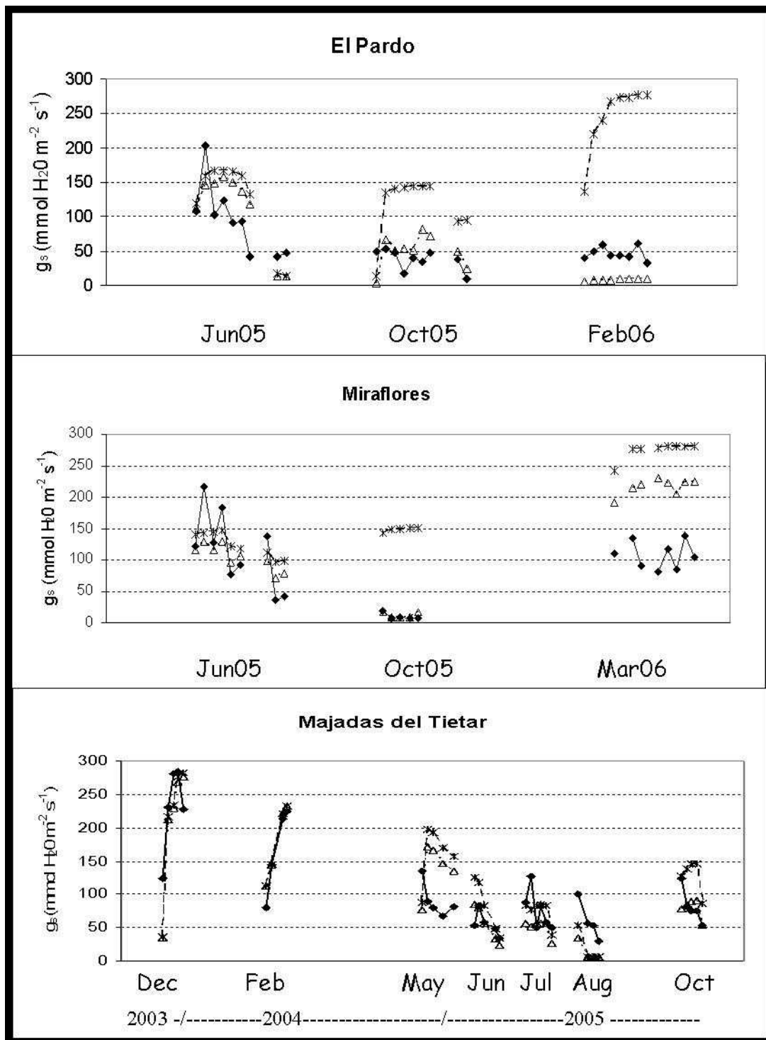
FIGURE 2. Validation of the g_s model for Q. ilex using measured data at El Pardo and Miraflores during the period June 2005 through March 2006 and at Majadas del Tietar December 2003 through October 2005. ♦, measured data; *, calculated data based on literature review parameterization; Δ, calculated data based on literature review parameterization including f_{\text{SMD}} function.
