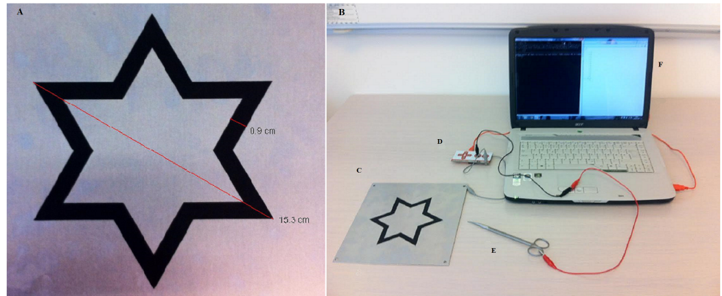
Figure 1 The test setup. Picture (A) shows detailed measurements and dimensions of the metal plate with the star-shaped track. Picture B shows a complete setup of the test with all its components. (C) Shows the star-shaped track used in the test. (D) Shows the The MakeyMakey. (E) Shows the standard Metzenbaum surgical scissors and (F) shows the computer running the software Star Track 32bit.exe. Photographs by Niels Kildebro.
