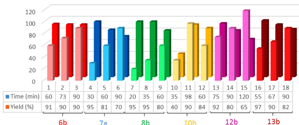
Fig. 9. Reusability of the catalyst in the synthesis of 1,2,4-triazoloquinazolinones (6b, 7a, 8b), 1,2,4-triazolo[4,3-a]pyrimidines (10b), pyrido[4,5-b]quinolone (12b) and pyrido[2,3-d]pyrimidines (13b).
