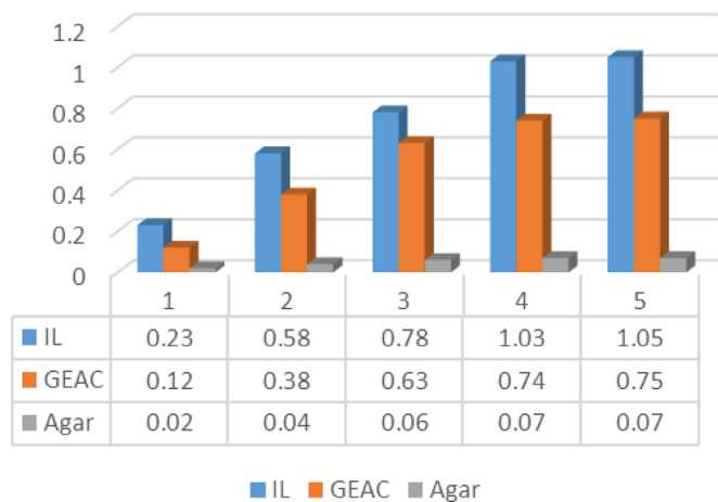
Fig. 8. A comparison between moisture resistant property of agar, IL, and agar-entrapped IL.
