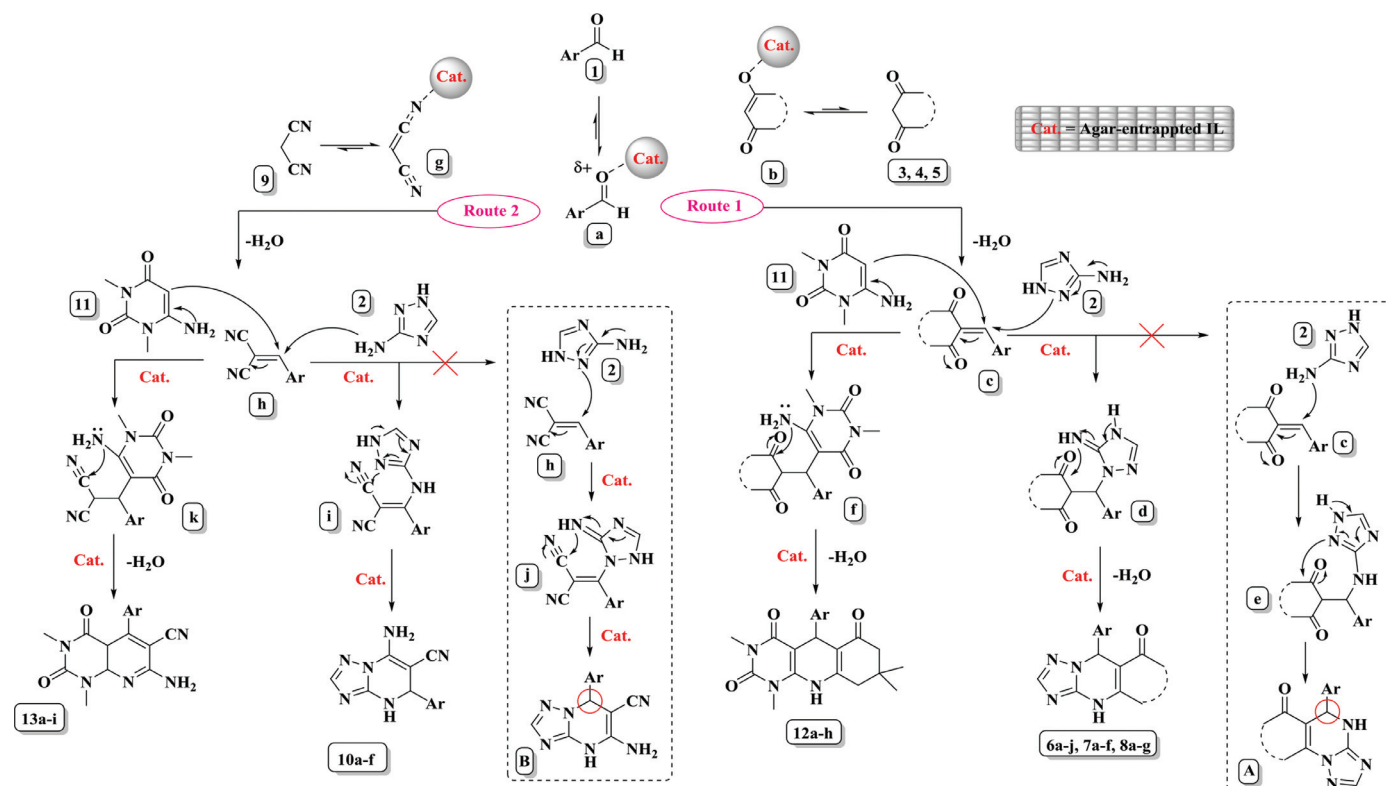
Scheme 2. The hypothesized mechanism for the synthesis of 1,2,4-triazolo[4,3- a ]pyrimidine, pyrido[2,3- d ]pyrimidine and pyrido[4,5- b ]pyrimidine, and 1,2,4-triazoloquinazolinone derivatives in the presence of agar-entrapped IL.
