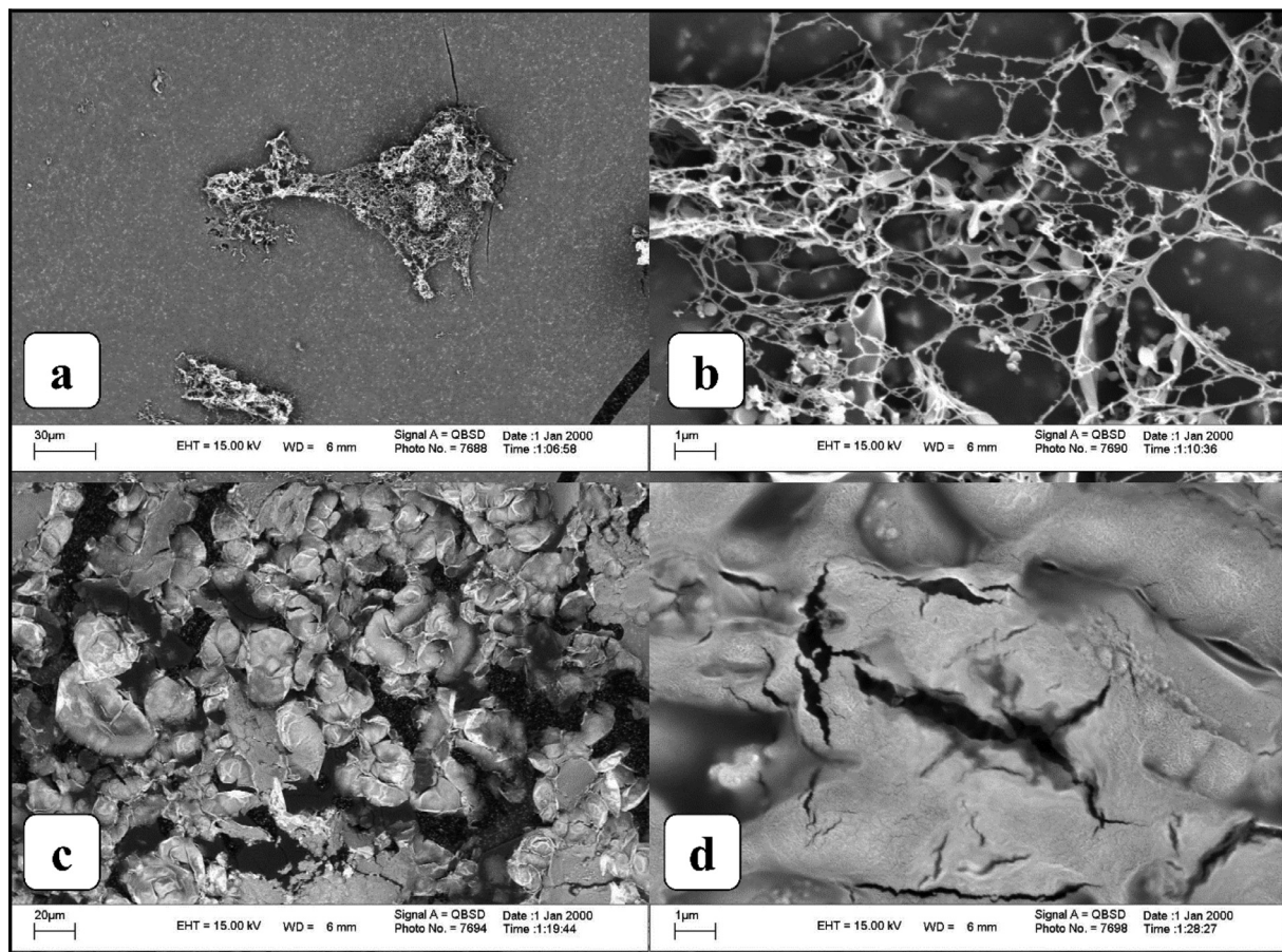
Fig. 6. SEM of DABCO (a and b) and agar-entrapped IL (c and d).
