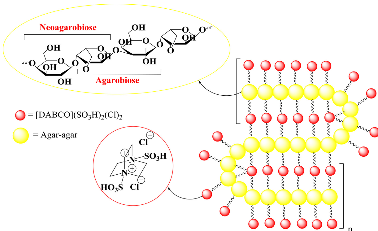
Fig. 1. Agar/agarose structure and agar-entrapped sulfonated DABCO.
