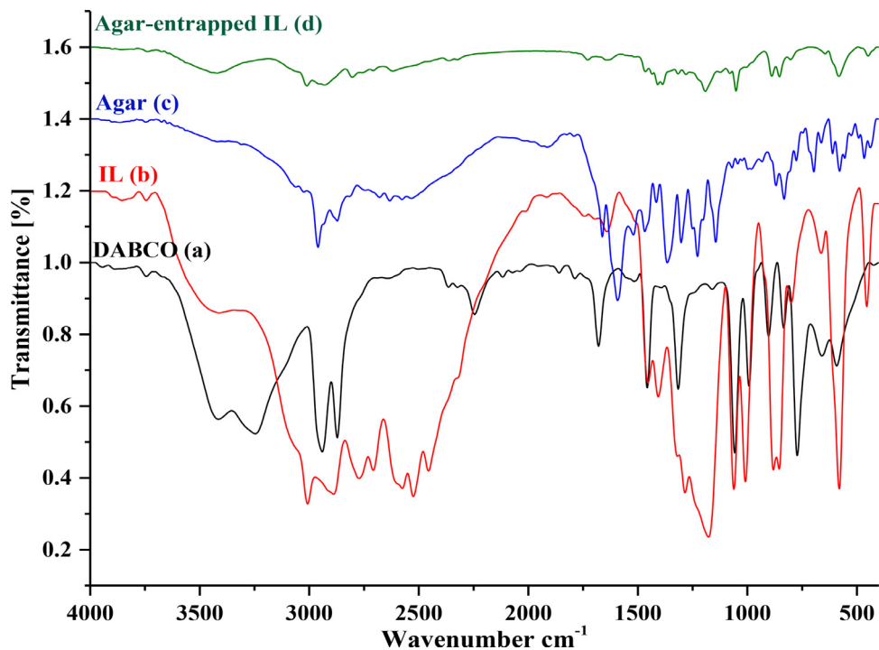
Fig. 5. FT-IR spectra of DABCO (a), [DABCO] ( \text{SO}_3\text{H} ) _2\text{Cl}_2 (b), agar (c) and agar-entrapped IL (d).
