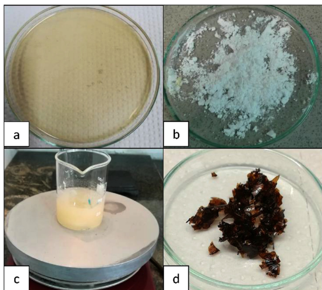
Fig. 3. Agar in heated water (a), [DABCO](SO 3 H) 2 (Cl) 2 (b), ionic liquid in warm water (c) and agar-entrapped ionic liquid (d).
