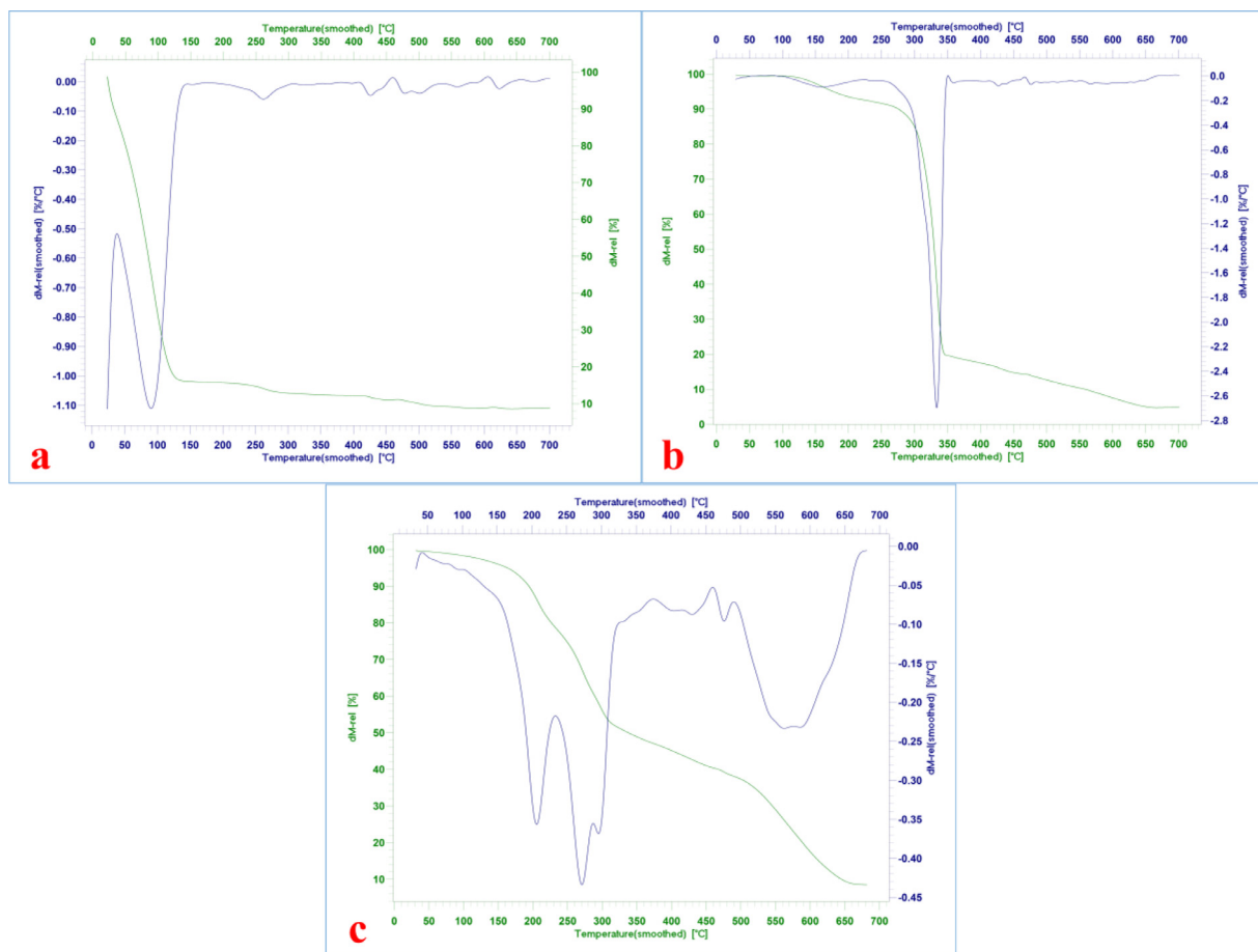
Fig. 7. TGA diagrams of agar (a) IL (b) and agar-entrapped IL (c).
