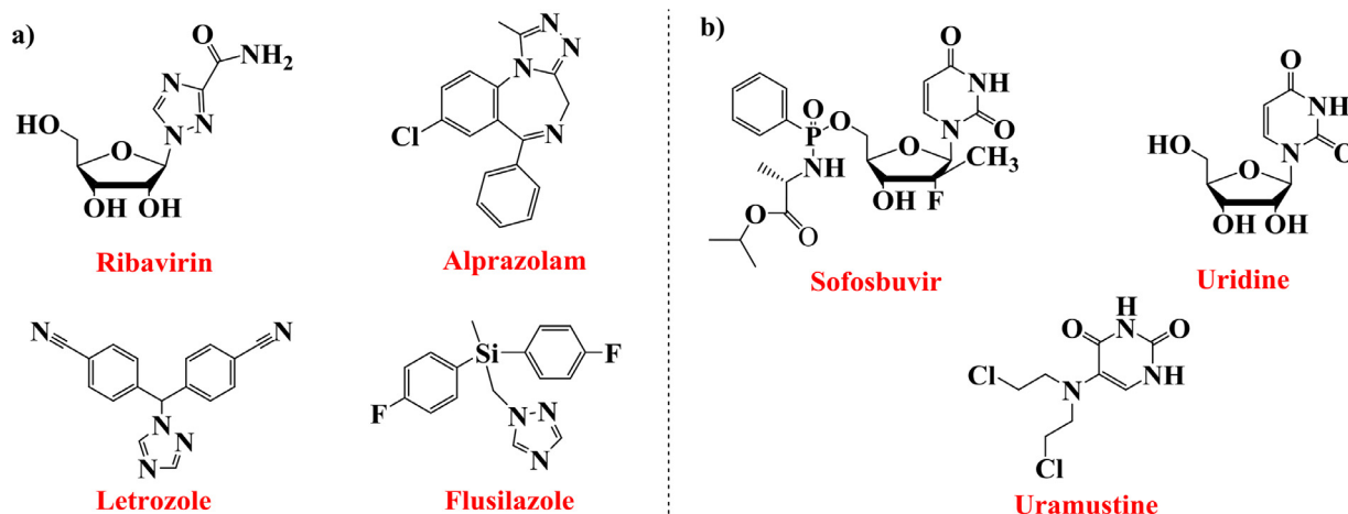
Fig. 2. The structures of some triazole (a) and uracil (b) containing drugs.
