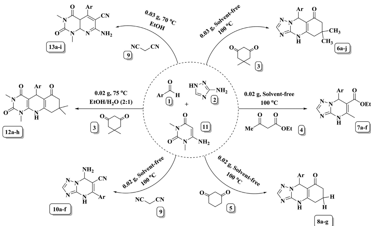
Scheme 1. Synthesis of 1,2,4-triazolo[4,3-a]pyrimidine, pyrido[2,3-d]pyrimidine and pyrido[4,5-b]pyrimidine, and 1,2,4-triazoloquinazolinone derivatives.
