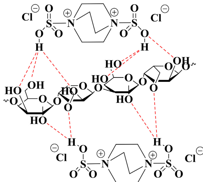
Fig. 4. Hydrogen bond probability of agar-entrapped IL.
