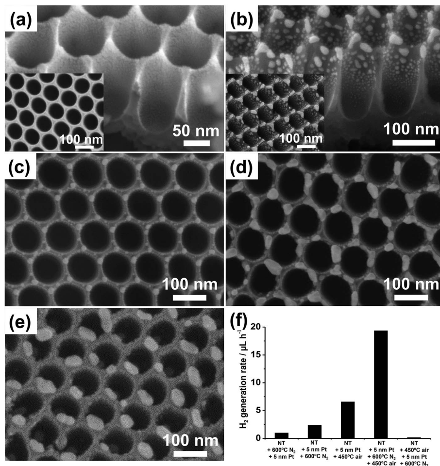
Fig. 11 (a–e) SEM images of \text{TiO}_2 nanocavity arrays: (a) sputter-coated with a 5 nm-thick Pt film and (b) after thermal dewetting in \text{N}_2 (600 °C); (c–e) sputter-coated with different Pt amounts ((c) 2, (d) 7, and (e) 10 nm) and then dewetted in \text{N}_2 . Insets in (a) and (b): top view SEM images. (f) Photocatalytic \text{H}_2 generation rate ( r_{\text{H}_2} ) of various Pt/ \text{TiO}_2 nanocavity arrays decorated by sputtering–dewetting of different Pt loadings. Fig. (a–f) are reprinted (adapted) with permission from ref. 139. Copyright 2016 American Chemical Society.
