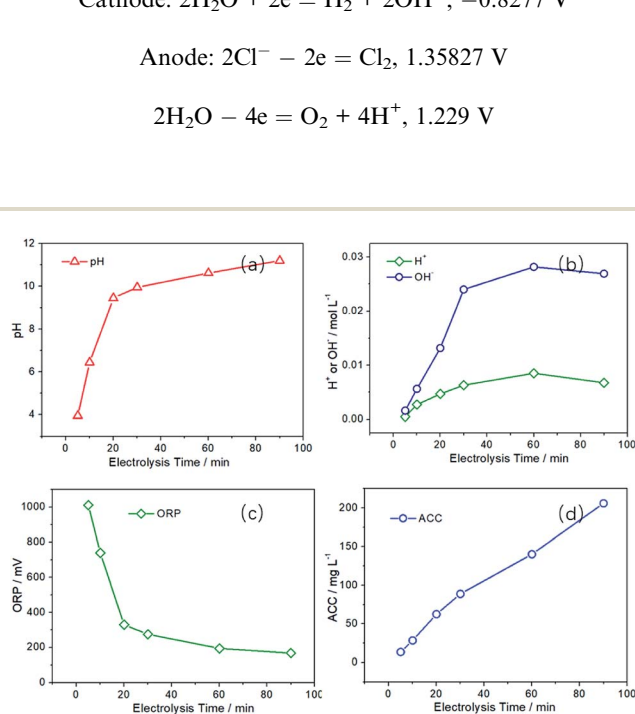
Fig. 6 Effect of electrolysis time on the pH, ORP and ACC values of SAEW and the content of H^+ and OH^- in anode and cathode region. ( i = 60 mA cm^{-2} , C_{NaCl} = 0.5 g L^{-1} ).
