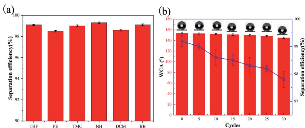
Fig. 12 (a) The separation efficiency of \text{SiO}_2\text{-S-PIH@ cotton} for various oil–water mixtures. (b) The variation of separation efficiency and WCA of \text{SiO}_2\text{-S-PIH@ cotton} versus the number of separation cycles.
