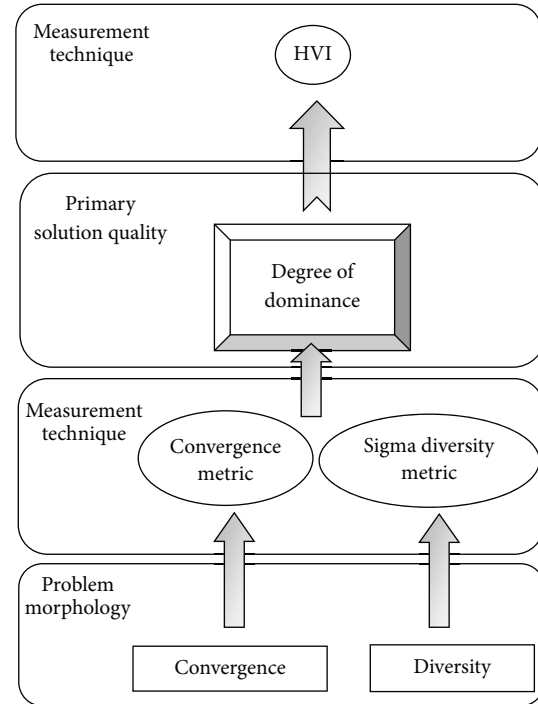
FIGURE 1: Hierarchy Axiom.
