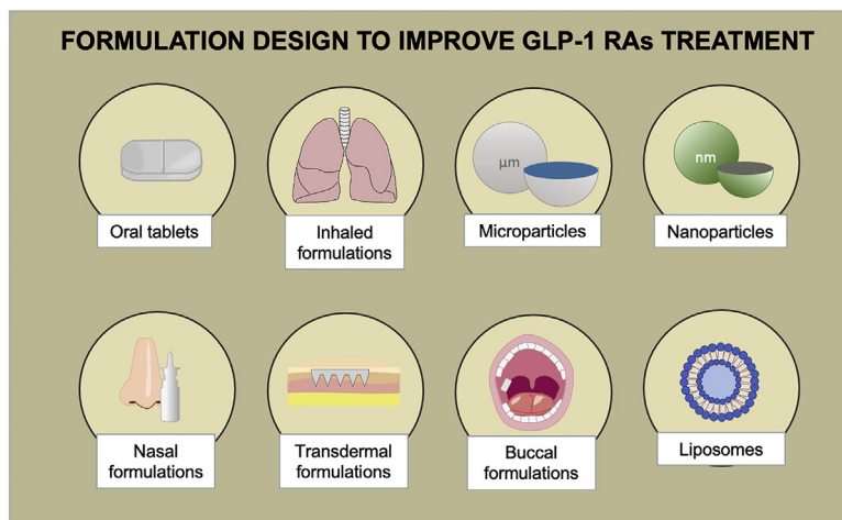
Figure 4 Formulation strategies for the administration of GLP1-RAs.
