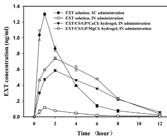
Figure 7 Exenatide blood levels vs. time profiles after subcutaneous (SC) or intranasal (IN) administration of exenatide (EXT) in solution or included in CaCl 2 or MgCl 2 hydrogels. Values are expressed as the mean ± SD ( n = 5). Figure reproduced and modified with permission from Ref. 72. Copyright © 2018 Elsevier B.V.
