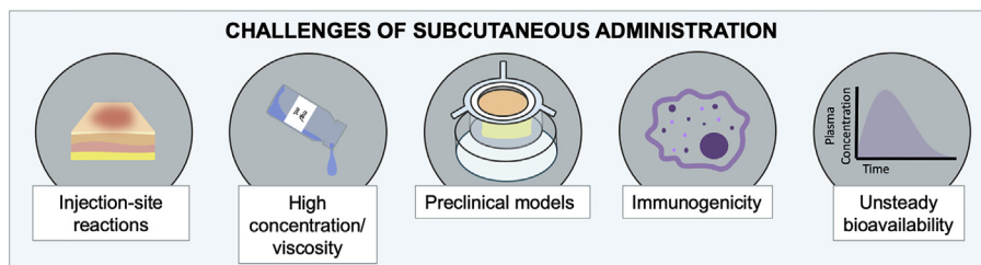
Figure 2 Challenges of subcutaneous administration of biotherapeutics.
