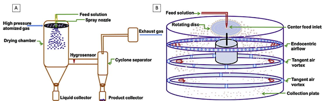
Figure 12 Schematic illustration of spray dryer (A) and ultrafine particle processing system (UPPS) (B) for the manufacture microparticles. Figure reproduced and modified with permission from Ref. 120. Copyright © 2015 Elsevier B.V.
