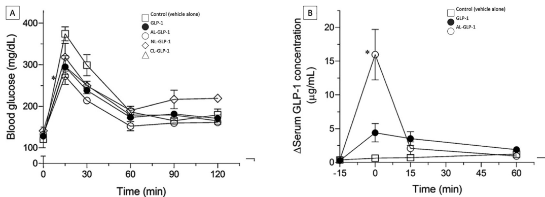
Figure 6 (A) Activity of GLP-1 formulations in an intraperitoneal glucose tolerance test in rats. (B) Serum GLP-1 concentrations in rats after intravenous administration of GLP-1 formulations. Figure reproduced and modified with permission from Ref. 68. Copyright © 2009 Elsevier B.V.
