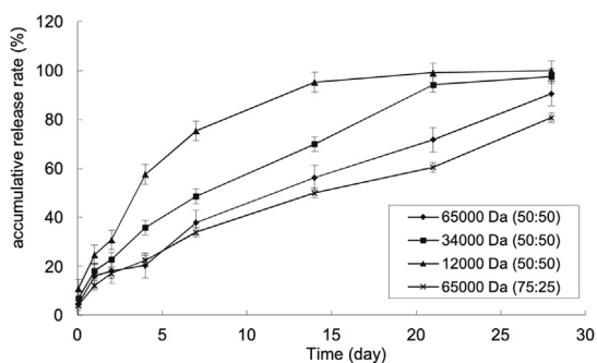
Figure 11 In vitro release profiles of exenatide loaded PLGA microspheres prepared with PLGA of different molecular weights and different copolymer compositions in HEPES buffer pH 7.4. Figure reproduced and modified with permission from Ref. 118. Copyright © 2013 Elsevier B.V.
