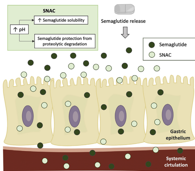
Figure 5 SNAC effect on the oral absorption of semaglutide. SNAC enhances the transcellular absorption of semaglutide by increasing the pH.
