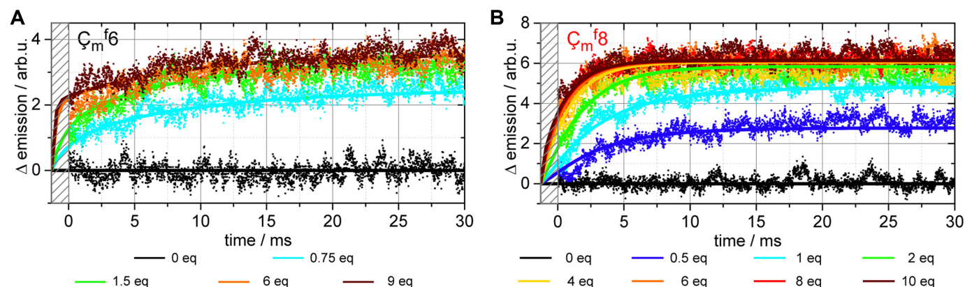
Figure 11. (A) Transient fluorescence signals after stopped-flow mixing of (A) 2.7 \mu\text{M } C_m^f6 and (B) 4 \mu\text{M } C_m^f8 with different concentrations of neomycin (indicated as equivalents of the aptamer concentration). The data are shown as points while the fits for a two-step model are displayed as solid lines.
