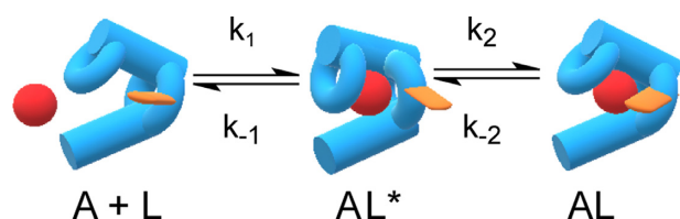
Figure 12. Cartoon of the proposed two-step binding model. The ligand is depicted as red sphere, the label as orange plate and the aptamer as blue clamp. A = aptamer, L = ligand, AL* = ligand bound intermediate state, AL = final, ligand bound state, k_n = rate of reaction step n , k_{-n} = back-rate of reaction step n .
