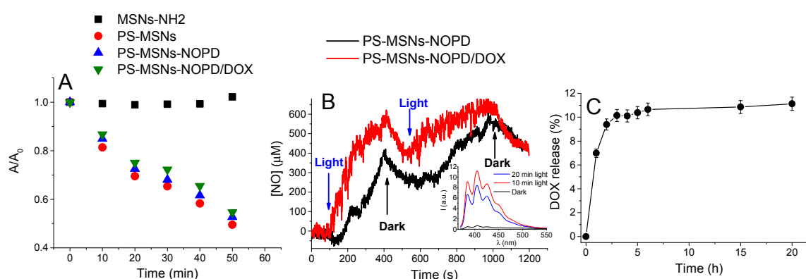
Figure 5. (A) A/A 0 ratio at 440 nm of p -nitrosodimethylaniline/histidine (RNO) (17 \mu\text{M} ) observed upon irradiation at 532 nm (50 mW) in the presence of different suspensions (1 mg mL -1 ) of MSNs in PBS (pH 7.4, 10 mM). (B) NO release profile observed upon irradiation at 405 nm (100 mW) of different suspensions (1 mg mL -1 ) of MSNs in PBS (pH 7.4, 10 mM). The inset shows the indirect e NO fluorimetric detection ( \lambda_{\text{exc}} = 365 nm) (see experimental) observed for PS-MSNs-NOPD suspension (1 mg mL -1 ) in the dark and after 10 and 20 min irradiation at 405 nm. (C) DOX release observed for PS-MSNs-NOPD/DOX suspension (1 mg mL -1 ) in PBS (pH 7.4, 10 mM) at 37 °C.
