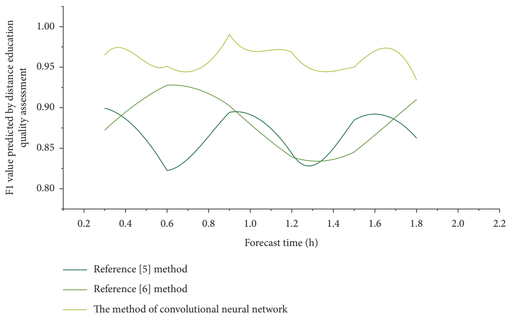
FIGURE 7: F1 value predicted by distance education quality assessment of three algorithms.
