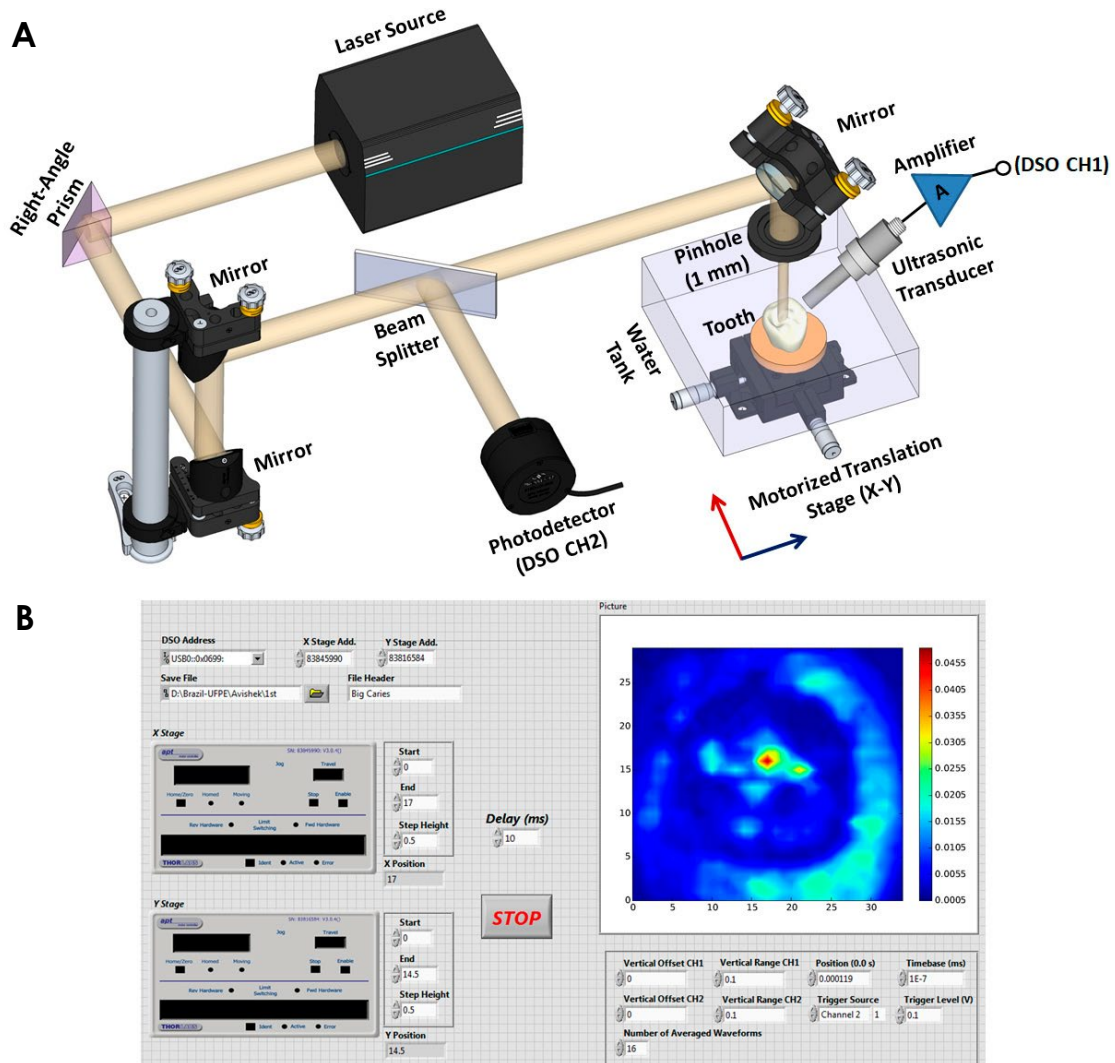
Fig. 1. A. Schematic diagram of the lab-made photoacoustic imaging system. B. Data acquisition and image reconstruction program in LabVIEW.
