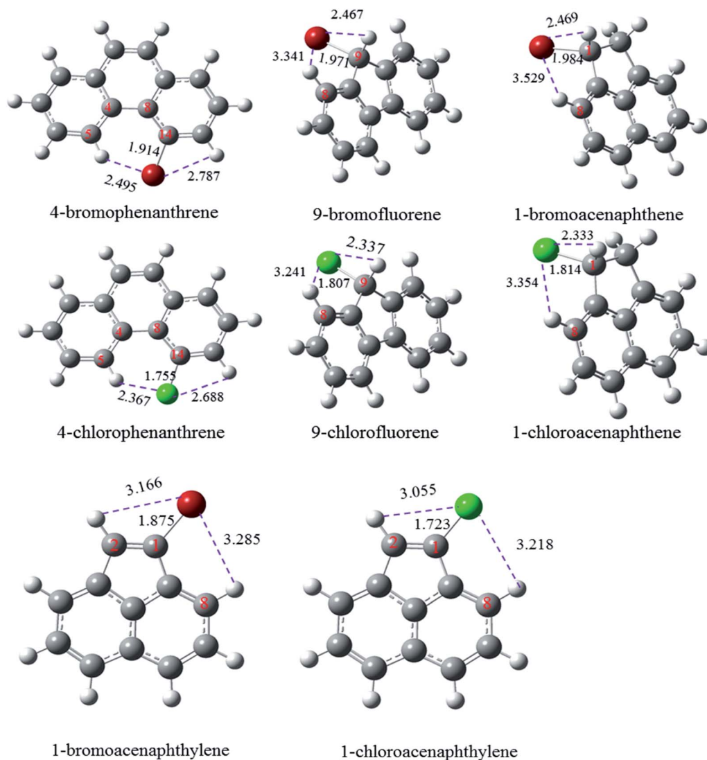
Fig. 3 Optimized structures of 4-halogenated phenanthrene, 9-halogenated fluorene, and 1-halogenated acenaphthene at the M06-2X/6-311++G(d, p) level.
