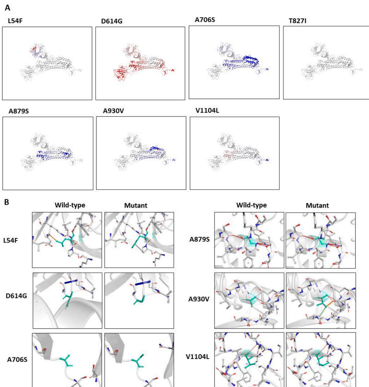
Fig. 3. Prediction of mutation impact on structural integrity of Spike glycoprotein, A) Analysis of protein flexibility due to mutations in Spike glycoprotein. The blue color signifies rigidification of the structure and red represents gain in flexibility. B) Interatomic interactions in Spike glycoprotein- The molecular structure of wild-type and mutant amino acid are highlighted in light-green color. The surrounding residues that are making close contacts with the wild type and mutant residues are also highlighted. (For interpretation of the references to color in this figure legend, the reader is referred to the web version of this article.)
