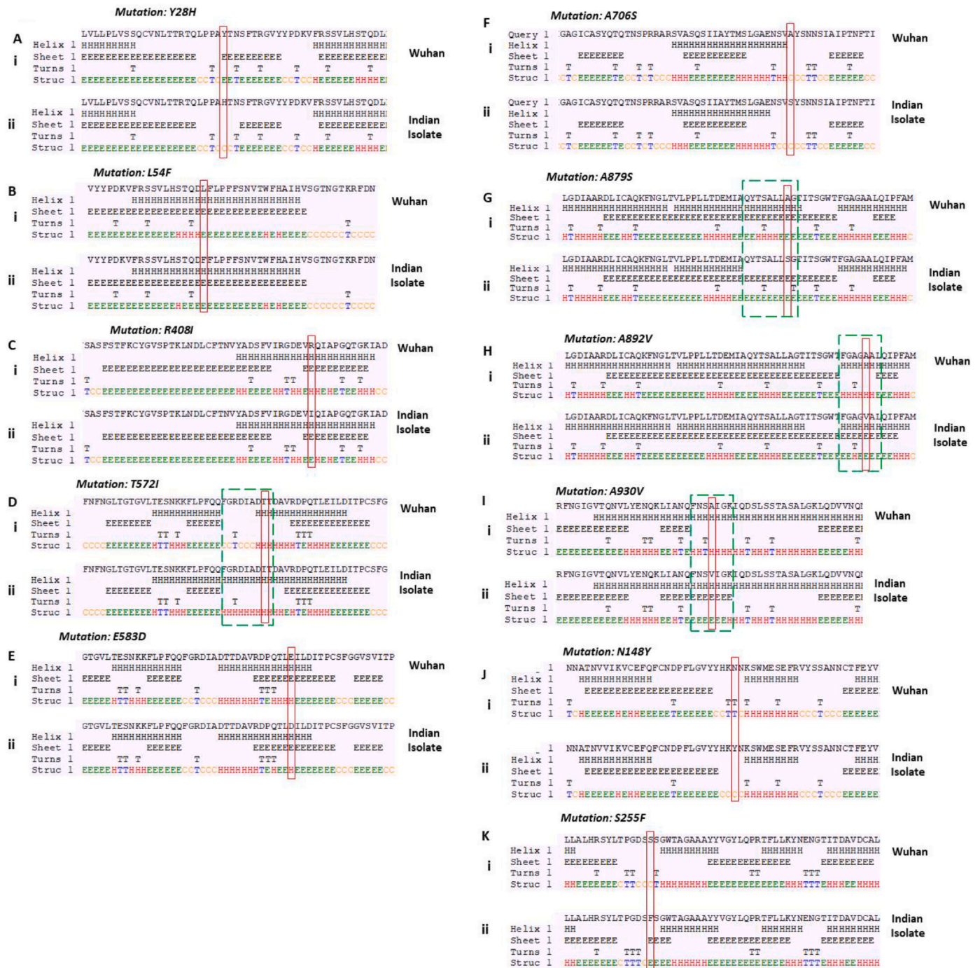
Fig. 2. Prediction of changes in the secondary structure of Spike glycoprotein due to mutations. Fig. A, B, C, D, E, F, G, H, I, J and K demonstrate mutations observed in Indian isolates. Panel (i) represents sequence of Wuhan isolate and panel (ii) represents sequence of Indian isolates. We observed a drastic change in the secondary structure between Wuhan and Indian isolates at four mutation sites as highlighted in the green box (Panel D, G, H and I). (For interpretation of the references to color in this figure legend, the reader is referred to the web version of this article.)
