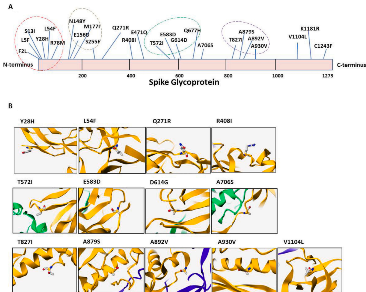
Fig. 1. A) The sequences of Spike glycoprotein obtained from India were aligned with the sequence from Wuhan (wet seafood market) SARS-CoV-2. The mutations were identified by amino acid sequence alignment by CLUSTAL Omega. The mutant residues are highlighted in the scheme of Spike glycoprotein. The Spike glycoprotein sequence of Wuhan SARS-CoV-2 was used as reference. The dotted circle represents mutation clusters. B) The location of mutant amino acids in the secondary structure of the Spike glycoprotein. The position of each amino acid mutation is highlighted as sticks in their respective panels.
