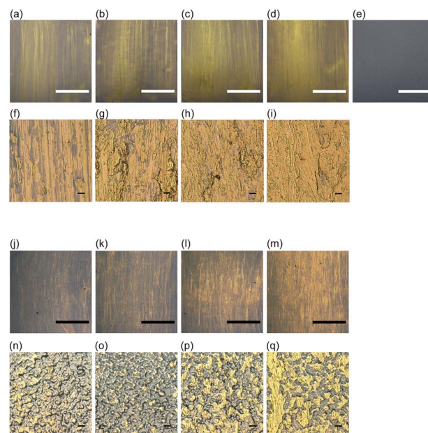
Fig. 2 Low-magnification (a–d, j–m) and high-magnification (f–i, n–q) digital microscope images of the O3MeOT layers prepared by rubbing at linear pressures of 40 \text{ gf mm}^{-1} (a–d, f–i) and 20 \text{ gf mm}^{-1} (j–q). Panel (e) shows a low-magnification image of the substrate. The scale bars in the low-magnification images (a–e, j–m) and high-magnification images (f–i, n–q) correspond to 10 mm and 10 \mu\text{m} , respectively.
