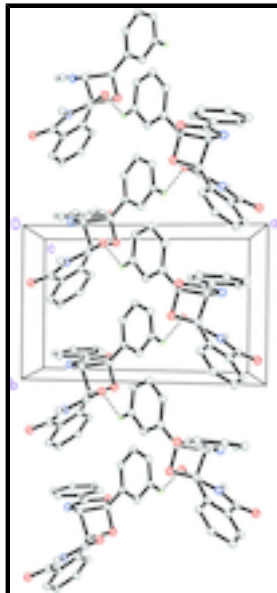
Fig. 2. The crystal structure of the title compound, viewed along the c axis, showing a hydrogen-bonded (dashed lines) chain along the b axis. H atoms not involved in the interactions have been omitted for clarity.
