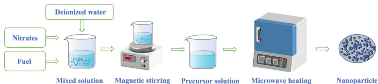
Fig. 3 Diagram of microwave induced combustion synthesis.
