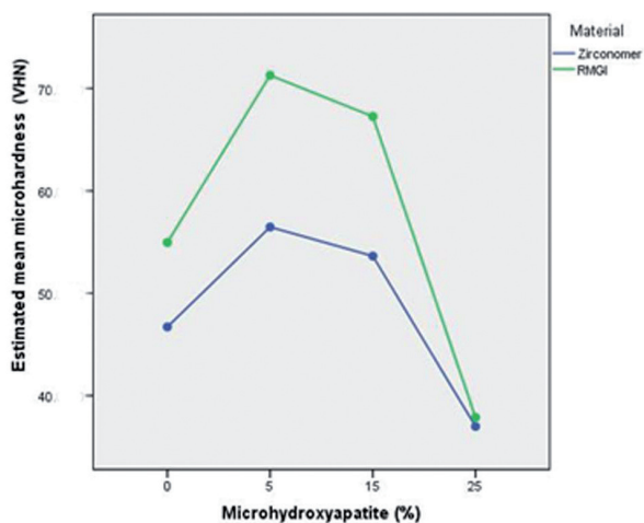
Fig. 3: Estimated mean Vickers microhardness values of Zirconomer and RMGI with adding 5%, 15% and 25% microhydroxyapatite.
