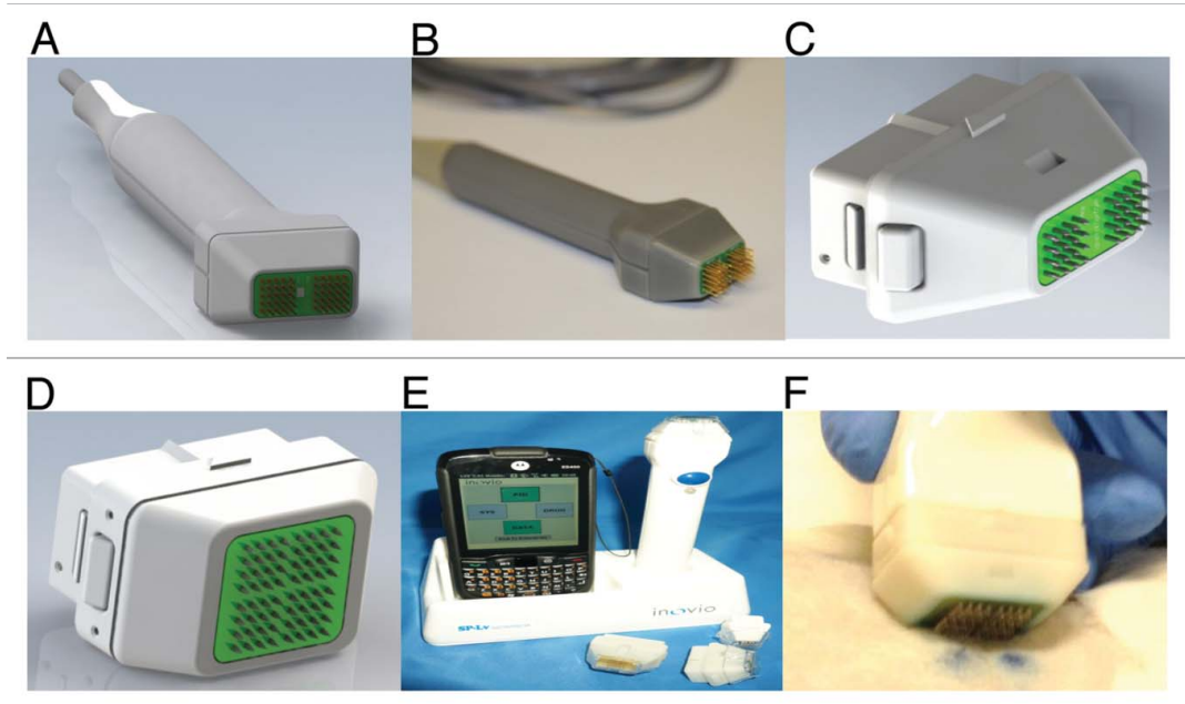
Figure 1. Multi-head device (A) CAD concept drawing of multi-head hand piece (B) Working prototype of 4×4 array with 1.5mm spacing. (C) Close up of CAD concept disposable 2-head array (m2SEP). (D) Close up of CAD concept 4-disposable head array (m4SEP). (E) Wireless device in base station with Pocket PC displaying the user interface. (F) The m4SEP in use in a guinea pig model.
