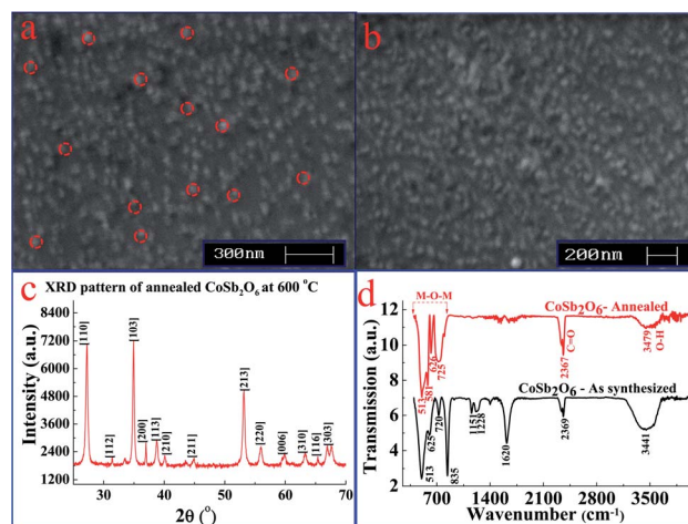
Fig. 2 (a and b) SEM images of annealed \text{CoSb}_2\text{O}_6 film at two different magnifications (dotted circles indicate the nanospheres used for the size calculation), (c) XRD pattern of \text{CoSb}_2\text{O}_6 annealed at 600^\circ\text{C} , and (d) FT-IR spectra of the as-synthesized (pre-annealed) and \text{CoSb}_2\text{O}_6 annealed at 600^\circ\text{C} .
