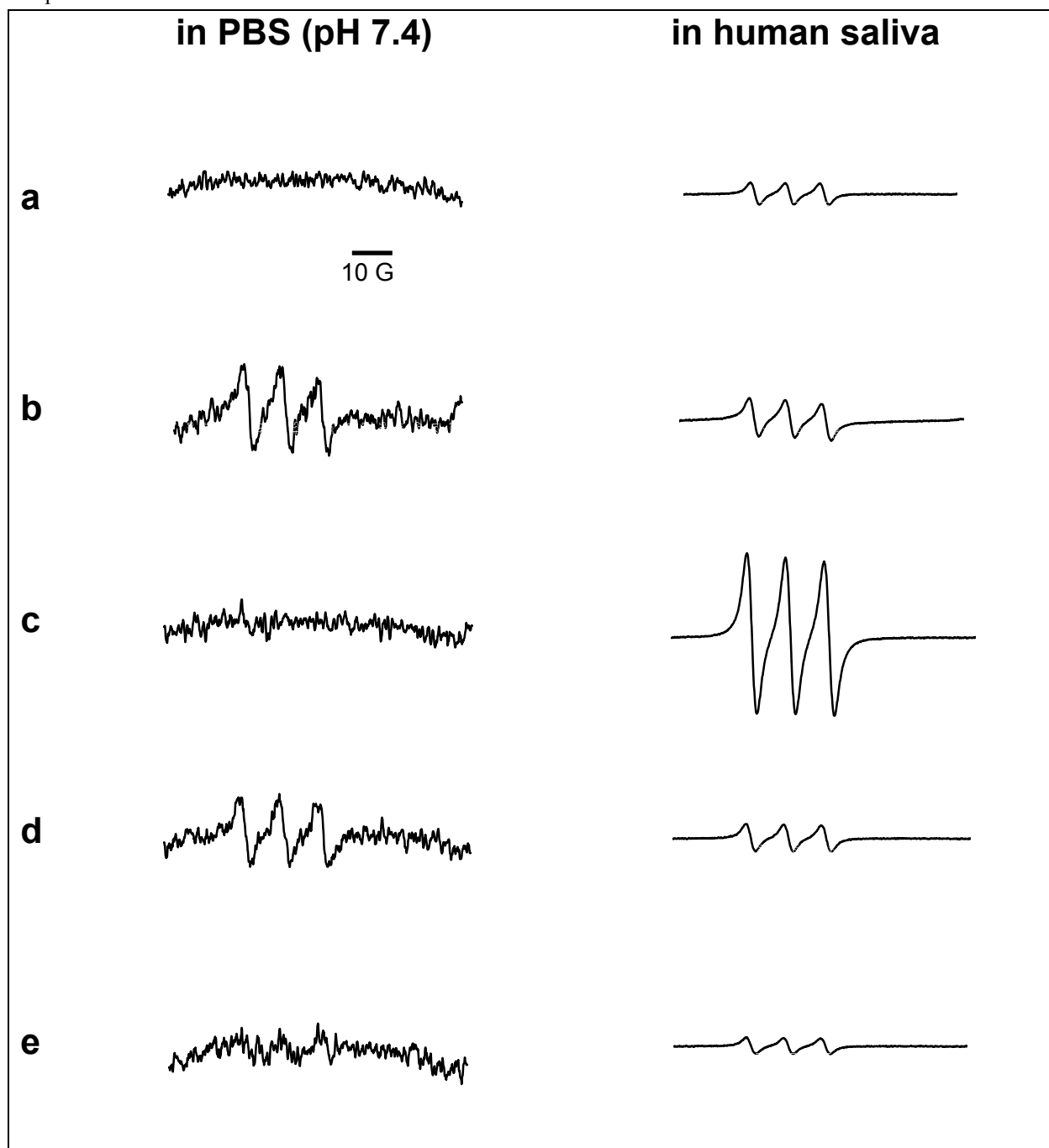
Figure 1. EPR spectra of the \cdot\text{NO-Fe}(\text{MGD})_2 spin adduct formed from the release of \cdot\text{NO} from tobacco xenobiotics in phosphate buffered-saline at pH 7.4 (left column) and human saliva (right column). The hyperfine splitting value, a_N , of these spectra is 12.4 G and the isotropic nuclear g value, g_{\text{iso}} , is 2.04. (a) 500 \mu\text{L} phosphate buffered saline (left column) or whole human saliva (right column); (b) 500 \mu\text{L} of a 1:1 w/v extract of smokeless tobacco; (c) 3.48 M (26.7 \mu\text{G} ) nicotine; (d) 1.1 M (10 mg) nitrosonornicotine (NNN); and (e) 1.0 M (10 mg) 4-(methyl-N-nitrosamino)-1-(3-pyridyl)-1-butanone (NNK). Each spectrum represents 15 summed signal acquisitions acquired using a receiver gain of 2 \times 10^4 and modulation amplitude of 1 G. The ordinate scale is \pm 1 \times 10^3 arbitrary units for all spectra in whole human saliva.
