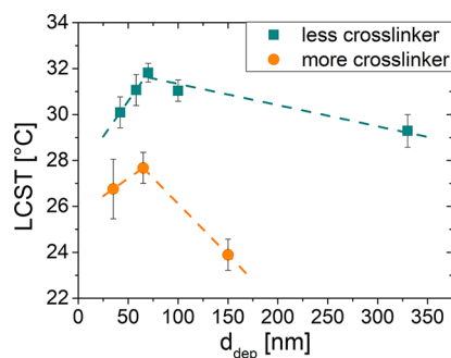
Figure 4. LCST as a function of deposited film thickness ( d_{\text{dep}} ) for differently cross-linked p(NIPAAm-co-DEGDVE) thin films (dotted lines are for guidance of the eye).
