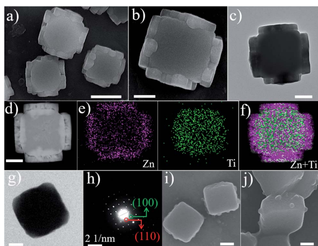
Fig. 3 (a and b) SEM images, (c) TEM image, (d) STEM image, and (e and f) elemental mapping images of \text{bMIL-125@ZIF-8} ; (g) TEM image and (h) SAED patterns of \text{bMIL-125} . (i and j) SEM images of the sample after growth of ZIF-8 on \text{bMIL-125} for 2 min. The scale bars are 500 nm (a), 200 nm (b, c, d, i, and j) and 100 nm (g).
