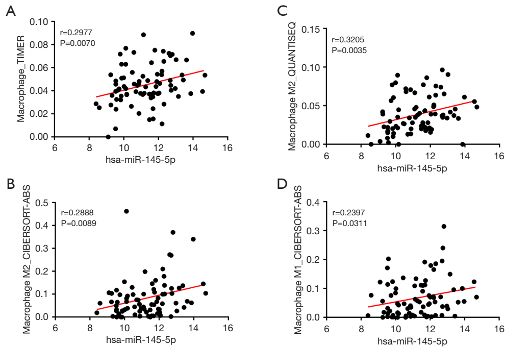
Figure 10 Correlation between miR-145-5p and macrophage infiltration level. (A) Macrophages_TIMER ( r=0.2977 , P=0.0070 ). (B) Macrophages M2_CIBERSORT-ABS ( r=0.2888 , P=0.0089 ). (C) Macrophages M2_QUANTISEQ ( r=0.3205 , P=0.0035 ). (D) Macrophages M1_CIBERSORT-ABS ( r=0.2397 , P=0.0311 ).
