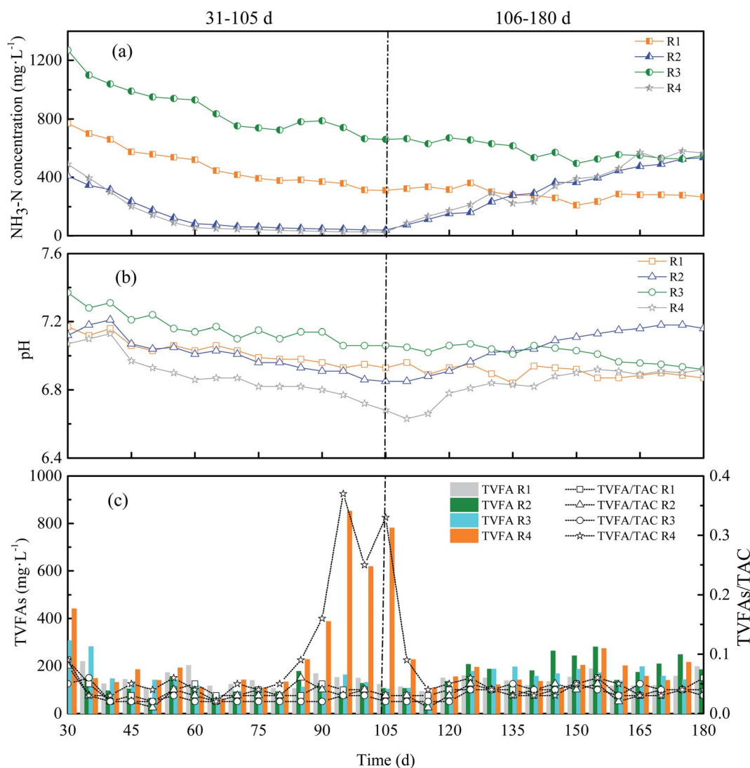
Fig. 3 \text{NH}_3\text{-N} concentration (a), pH (b), TVFAs and TVFAs/TAC (c) of four reactors with different KNPSs.
