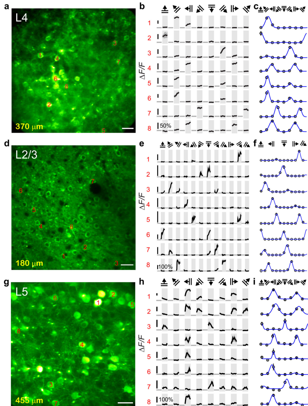
Fig. 3. Characterization of tuning properties of L4, L2/3, and L5 neurons in V1 (a) An example in vivo image of L4 neurons. Numbers label example somata. (b) Calcium transients \Delta F/F , and (c) tuning curves of the somata in a; Light gray background in b: 6-sec drifting grating (topmost labels) presentation; Dark gray shade in b and error bars in c: s.e.m.. (d–i) Example in vivo images, calcium transients, and tuning curves of (d–f) L2/3 and (g–i) L5 neurons. Scale bar: 25 \mu\text{m} . Representative results from 3 Scnn1a -Tg3-Cre (L4), 6 Thy1 -GCaMP6 GP4.3 (L2/3), and 5 Rbp4 -Cre (L5) mice.
