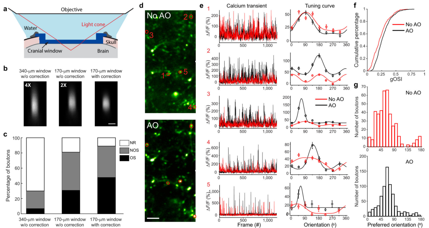
Figure 2. Adaptive optics is essential for tuning curve characterization
