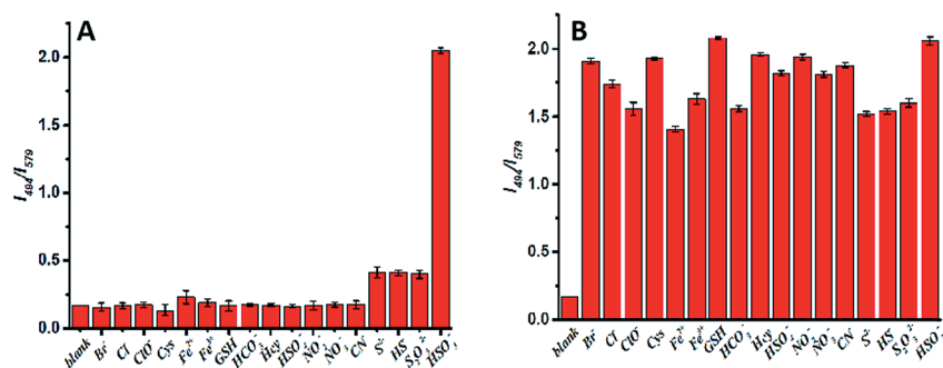
Fig. 3 (A) Relative fluorescence of IN-CZ ( I_{494}/I_{579} ) in the presence of various analytes. (B) Relative fluorescence of IN-CZ ( I_{494}/I_{579} ) towards NaHSO 3 (50 μM) when coexisting with various other analytes. (100 μM): Br - ; Cl - ; ClO - ; Hcy; Cys; GSH; HSO 4 2- ; HCO 3 - ; Fe 2+ ; Fe 3+ ; NO 2 - ; NO 3 - ; CN - ; S 2- ; HS - ; S 2 O 3 2- ; SO 3 2- /HSO 3 - (50 μM) (except: GSH 1 mM, Hcy 1 mM, Cys 1 mM) in PBS buffer solution (pH = 7.4, PBS = 10 mM, IN-CZ = 10 μM). Excitation at 420 nm.
