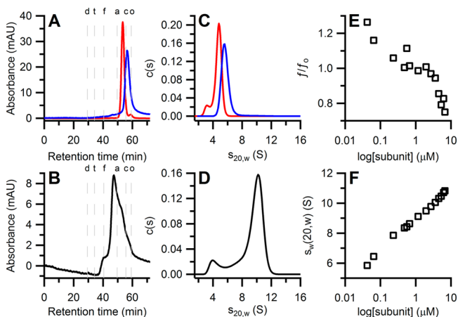
Figure 5. Biophysical characterization of the B. subtilis class Ib RNR (all at 1 μM) in the absence of nucleotides. (A) Overlaid SEC chromatograms of holo-Mn III 2 -Y· NrdF (red trace) and NrdE (blue trace). (B) SEC chromatogram of a 1:1 mixture of Mn III 2 -Y· NrdF:NrdE. Letters above the chromatograms indicate the retention time of molecular weight standards (d = Blue dextran 2000, t = thyroglobulin, f = ferritin, a = aldolase, c = conalbumin, o = ovalbumin). (C) Overlaid s 20,w distributions of holo-Mn III 2 -Y· NrdF (red trace) and NrdE (blue trace). (D) The s 20,w distribution of a 1:1 mixture of Fe III 2 -Y· NrdF:NrdE. (E) A plot of the weight averaged frictional ratios versus loading concentration of 1:1 mixture of Fe III 2 -Y· NrdF:NrdE shows a steep decrease as the subunit concentrations increase. 40 (F) An isotherm plotting the weight averaged s 20,w against loading concentration of 1:1 mixtures of Fe III 2 -Y· NrdF:NrdE indicates complicated quaternary structural dynamics of the B. subtilis class Ib RNR.
