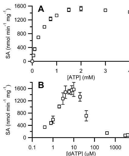
Figure 3. Effector nucleotide concentration-dependence of CDP reduction by a 1:1 mixture of \text{Mn}^{\text{III}}_2\text{-Y}\cdot NrdF and NrdE. Assays were conducted with 0.5 \mu\text{M} of each subunit. Error bars represent \pm 1 standard deviation from the mean. (A) Dependence of B. subtilis RNR activity on ATP. (B) Dependence of B. subtilis RNR activity on dATP.
