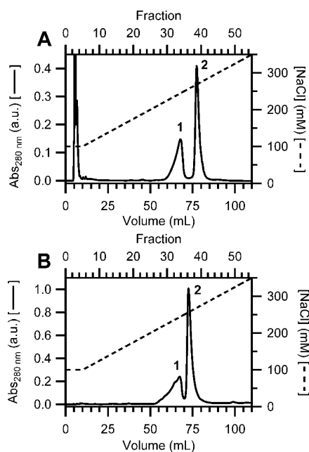
Figure 2. Separation of holo-Mn III 2 -Y· NrdF (A) and holo-Fe III 2 -Y· NrdF (B) from apo-/mis-metalated NrdFs by anion exchange chromatography on a MonoQ column. The material eluting in the void volume in (A) is NrdI ox . Peak 1 corresponds to apo-/mis-metalated NrdF and 2 to holo-Me III 2 -Y· NrdF.
