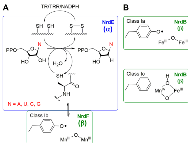
Figure 1. Ribonucleotide reduction catalyzed by class I RNRs. (A) The class Ib RNRs are composed of NrdE ( \alpha ) and NrdF ( \beta ) which are proposed to form an \alpha_2\beta_2 complex during substrate turnover (only one \alpha/\beta pair depicted). The stable dimanganic-Y housed in \beta ( 1 Y/\beta_2 ) oxidizes an essential Cys residue in the active site of \alpha to a thiyl radical through a long-range radical transfer process involving redox-active amino acids in both subunits. Reduction of NDPs to dNDPs occurs concomitant with oxidation of two Cys residues to a disulfide. The disulfide is rereduced by a thioredoxin (TR) or NrdH (a glutaredoxin-like thioredoxin), thioredoxin reductase (TRR), and NADPH. (B) The dimetallo-cofactors of the class Ia and Ic \beta subunits.
