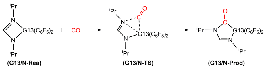
Scheme 2 Mechanism for catching reaction of CO by G13/N-based FLP.
