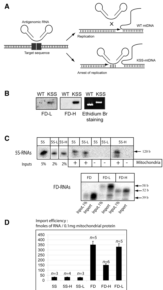
Figure 2. (A) Scheme of the anti-genomic strategy. (B) Southern hybridization of wild-type or KSS mtDNA fragments with labeled recombinant RNAs (FD-L and FD-H) at 37^\circ C . (C) In vitro import of the recombinant RNAs. Autoradiography of isolated mitochondria RNA separated in denaturing 10% PAAG is presented; 5S rRNA derived molecules above and FD-RNA derived ones below. The size of RNA molecules is shown at the right. 'Input', 1–5% of RNA used for each assay, representing 30–150 fmols of labeled RNA. Mitochondria (+) corresponds to the import assay, Mitochondria (–) to the mock import assay without mitochondria, used as a control for non-specific protein–RNA aggregation. (D) The import efficiencies, expressed in fmols of protected RNA to 0.1 mg of mitochondrial protein, as described elsewhere (32); n , number of independent experiments; n = 3 –6, as detailed upon each graph.
