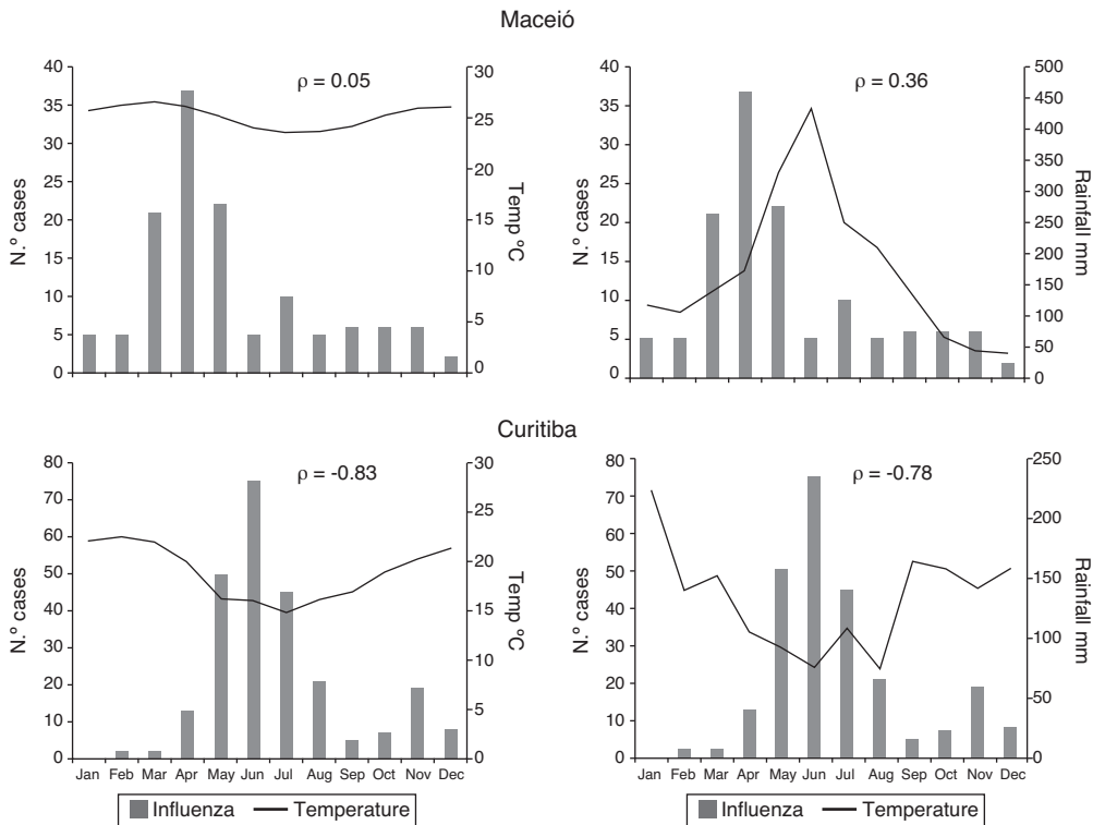
Fig. 4 – Spearman correlation analysis between monthly temperature and rainfall with influenza detection in the cities of Maceió and Curitiba, 2000–2010.
