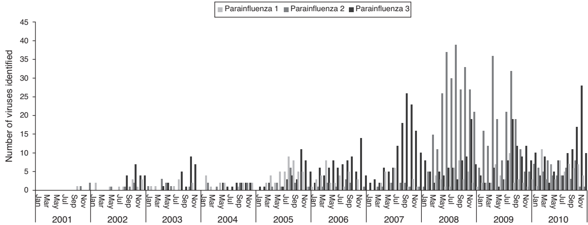
Fig. 3 – Circulation of parainfluenza viruses detected in the sentinel units, Brazil, 2001–2010.
