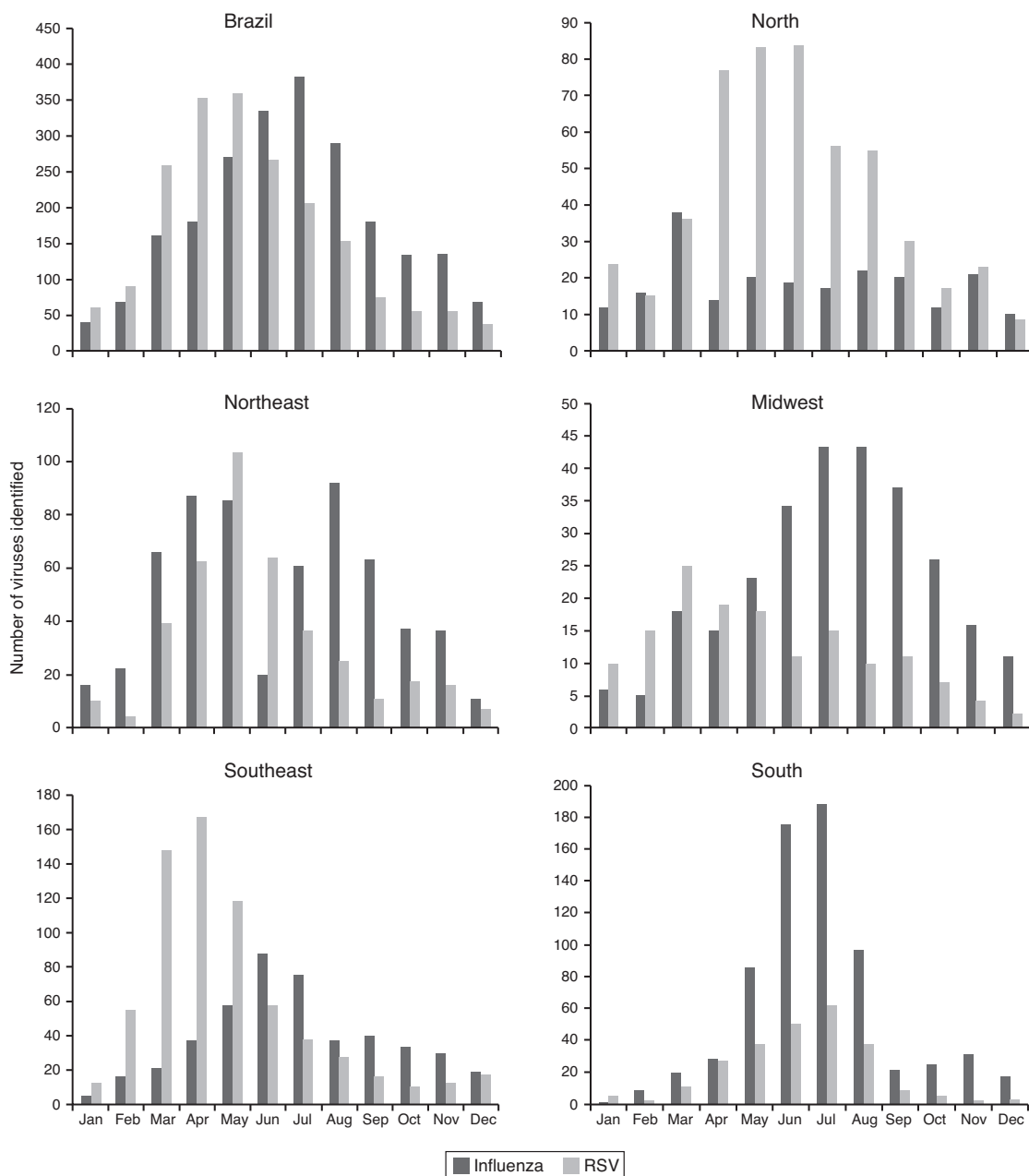
Fig. 2 – Number of influenza virus and respiratory syncytial virus (RSV) identified in the sentinel units per month in Brazil and in its five regions, 2000–2010.
