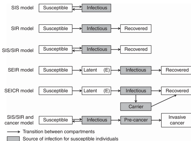
Figure 1. Transmission models represented as flow diagrams. Some examples of alternative compartmental models for modelling infectious diseases. The total population is distributed into mutually exclusive epidemiological compartments. The models are defined by these compartments and the possible transitions between them. In the simplest models, there are two or three states: susceptible, infectious, and recovered. More complex models can also account for a latent infection, and carrier status. Finally, transmission and carcinogenic phases of the natural history of infection-related cancers can be combined into a single model.
