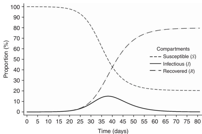
Figure 2. Epidemic dynamics of the SIR model in a closed population. The evolution of a SIR model over time is depicted by the curves representing the proportion of susceptible, infectious, and recovered individuals of the population. In this example, the epidemic peaks with 15% of the population in the infectious state at 37 days. By the end of the epidemic, 80% of the population has recovered and 20% is still susceptible, never having been infected.
