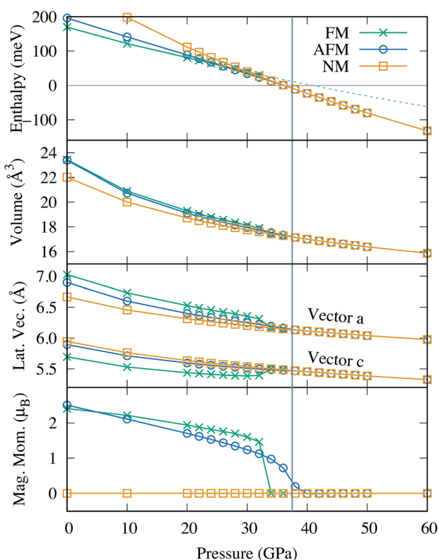
Fig. 3 The top panel shows the formation enthalpy of FeBi 2 in the FM, AFM and NM configuration (in meV per atom). The dashed line serves as a guide to the eye and was obtained from a quadratic fit to the enthalpy of the FM state between 0 and 30 GPa, before the magnetic collapse. The second panel shows how the volume per atom evolves as a function of pressure for the three spin configurations, whereas the third panel illustrates how the lattice vectors change. The magnetic moment per Fe as a function of pressure is shown in the bottom panel. The vertical gray line denotes the transition pressure above which FeBi 2 becomes thermodynamically stable.
