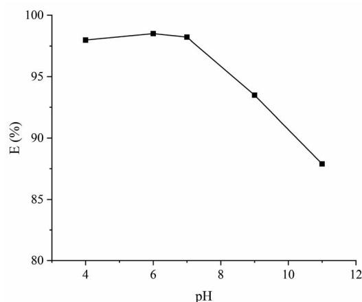
Fig. 7 Effect of pH for CR removal.
