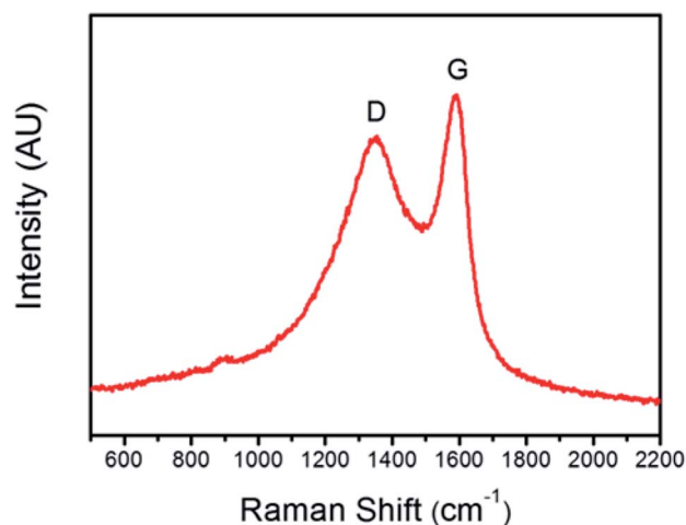
Fig. 4 Raman spectrum of carbonized cotton (CC) fibers.
