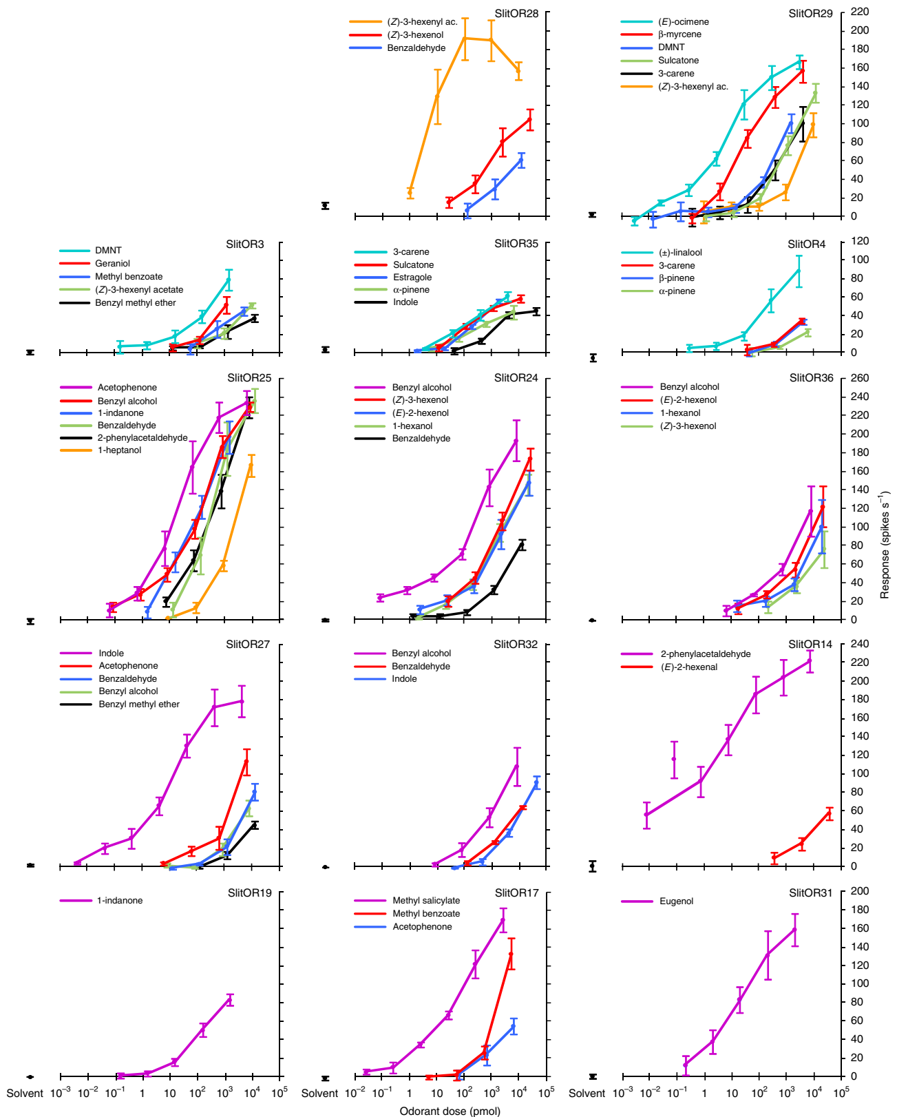
Figure 3 | Dose-response analysis of SlitORs. Mean response of 14 SlitORs to a range of odorant doses. Odorant doses correspond to the amount of molecules (in pmol) flowing out of the stimulus cartridge, to compensate the differences of volatility and affinity to paraffin oil solvent between chemicals 33 . Error bars indicate s.e.m. ( n = 5 ). Responses to solvent are indicated in black. Only the six best ligands are represented for receptors on which more odorants have been tested.
