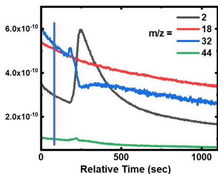
Fig. 8 Mass spectra of gas during treatment of neoprene with m/z = 2 for H_2 , 18 for H_2O , 32 for O_2 and 44 for CO_2 . The vertical line corresponds to the insertion of sample after a stabilization time of the atmosphere.
