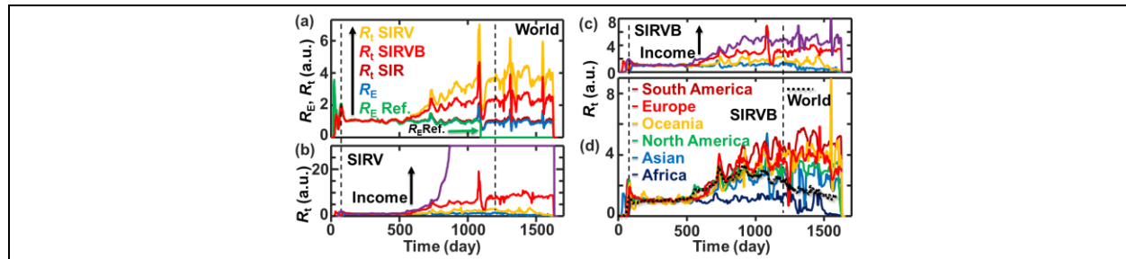
Figure 3. Reproduction number analysis of the world average data grouped and summarized in the raw data by Mathieu et al. 24 (a) R_E and R_t values of different models for the world average data. The reference R_E values is taken from the raw data. R_t values of (b) SIRV model, (c) SIRVB model for the average of four groups of countries ordered from low to high incomes, and (d) SIRVB model for the countries in the six continents. Data are smoothed. The dashed lines are when WHO announced the start (March 11, 2020) and the end of the pandemic (May 5, 2023).
