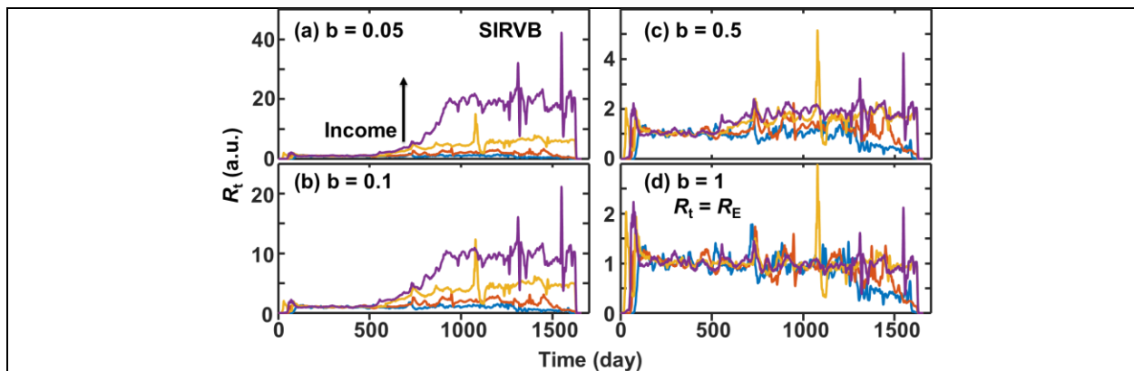
Figure 4. (a-d) The effect of breakthrough rate on the calculations of R_t values in the SIRVB model. The four groups of countries in the raw data with low to high incomes are used as examples. Curves of b = 0.2 have been shown in Figure 3c .
