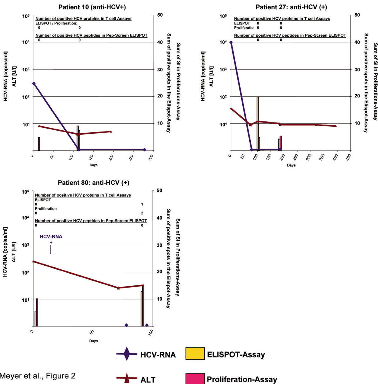
Figure 2 Biochemical, virological and immunological course of acute hepatitis C in asymptomatic patients with spontaneous clearance: patients who developed anti-HCV antibodies.
