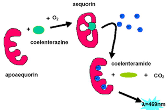
Fig. 1: Mechanism of light emission by aequorin upon Ca^{2+} -binding.
