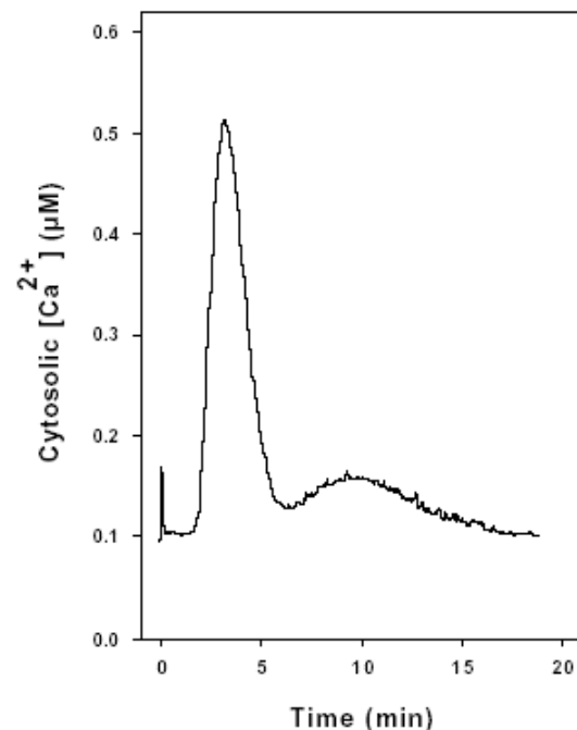
Fig. 3: Kinetics of the \beta -glucan elicitor-induced enhancement of the [Ca^{2+}]_{cyt} in soybean cells. \beta -Glucan fragments with the degree of polymerization of 7-15 (DP 7-15, 60 mM) were added at time = 0.
