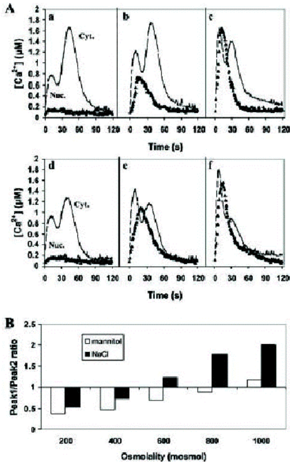
Fig. 6: Effect of the nature of the osmoticum and the strength of the hyper-osmotic shocks on the changes in nuclear and cytosolic calcium in tobacco BY-2 cells. Panel A: Calcium signatures monitored in BY-2 cells expressing apoaequorin either in the nucleus ( \blacktriangle ) or in the cytosol ( - ) in response to various hyper-osmotic treatments challenged with neutral (mannitol; traces a-c) or with saline osmoticum (NaCl; traces d-f). The variations of osmolality were 300 mosmol (traces a,d), 520 mosmol (traces b,e) and 880 mosmol (traces c,f). Panel B: Changes observed in the ratio of peak1/peak2 according to the strength and the nature of the osmoticum in independent experiments ( n=3 ). Reprinted from (14): Pauly et al. (2001), Cell Calcium 30:413-421 with permission of the publisher Churchill Livingstone.
