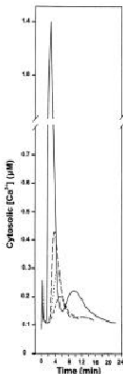
Fig. 4: Effect of the \text{Ca}^{2+} channel inhibitor \text{La}^{3+} on the \beta -glucan-induced [\text{Ca}^{2+}]_{\text{cyt}} response. \beta -Glucan was added at time = 0 (DP 7-15, 250 mM) alone (—) or after 2 min of preincubation with 2 mM \text{La}^{3+} (---), 4 mM \text{La}^{3+} (· · ·) or 6 mM \text{La}^{3+} (- - -).
