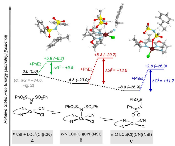
Fig. 3 Energy landscape for HAT in the reaction of \text{LCu}^{\text{II}}(\text{Cl})(\text{CN}) , \cdot\text{NSI} , and ethylbenzene. Gibbs free energies (enthalpies) [kcal mol -1 ] are computed at 298.15 K at the M06-D3(0)/basis-II/SMD(CH 2 Cl 2 )/M06-D3(0)/basis-I level of theory.
