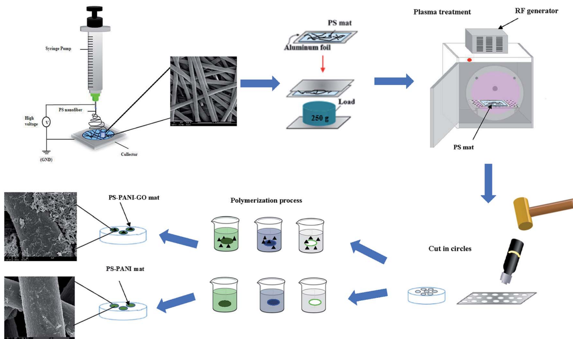
Fig. 1 Preparation steps followed to obtain flexible PANI and PANI, graphene on PS fibre mat.
