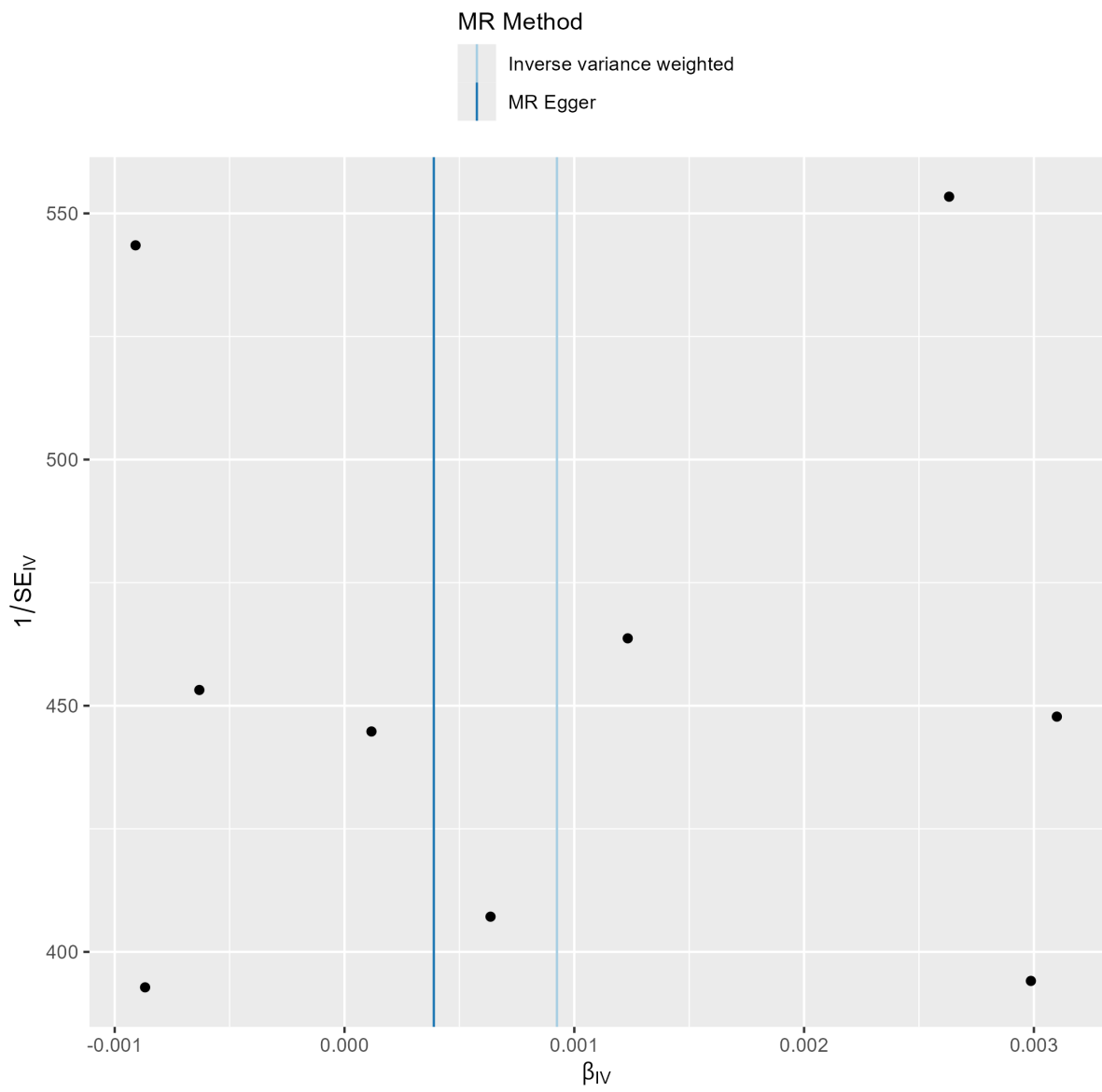
EH-LS funnel plot
