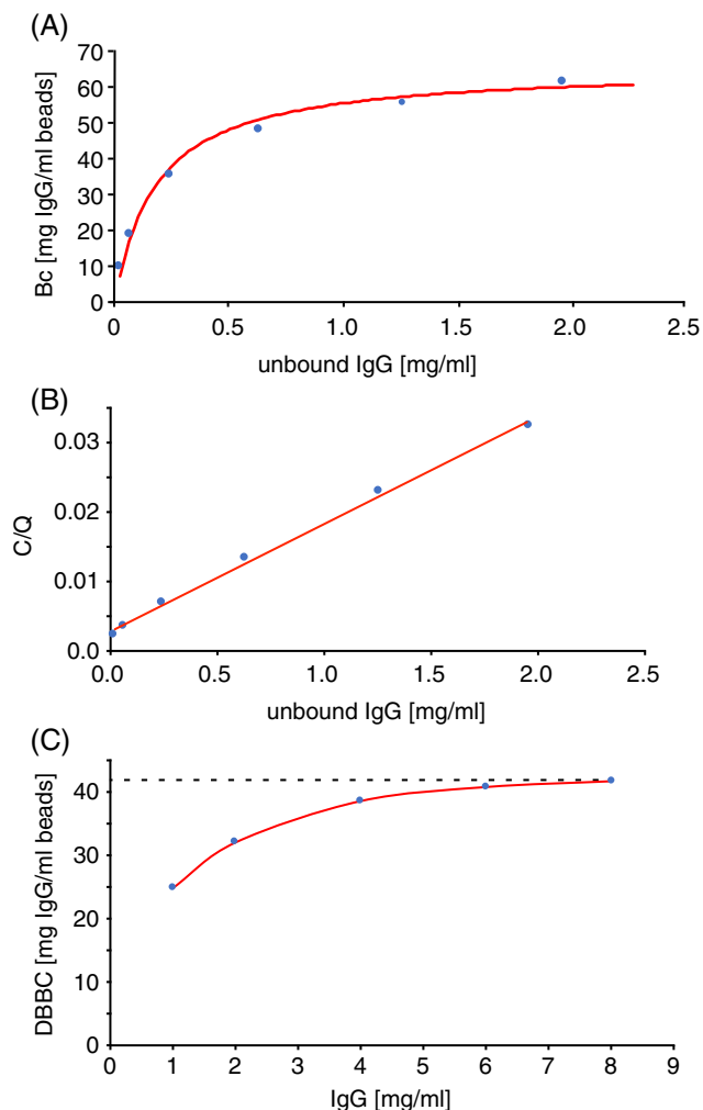
Figure 1. Capacity assays with a humanized mAb IgG1 on the magnetic protein A agarose beads, LOABeads PrtA. (A) Static binding capacity from adsorption equilibrium experiments fitted with Langmuir isotherm. (B) Linearized Langmuir isotherm (Hanes plot), to obtain the maximum binding capacity Q_{max} . r^2 = 0.9962 . (C) Dynamic bead binding capacity, defined as 90% load of antibody after 1-h residence time, DBBC_{1-h} , for different concentrations of monoclonal antibody.
