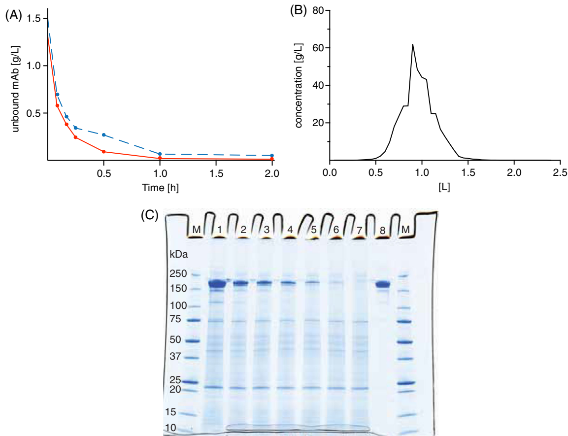
Figure 5. Pilot scale purification using non-clarified cell broth. (A) Adsorption efficiency from run B1, 15.73 L (red/solid), and run B2, 16.25 L (blue/dashed), with mAb concentrations of 1.31 and 1.51 g/L, respectively, using 0.8 and 1 L magnetic beads. (B) Elution profile from run B2, as measured at A_{280} . (C) Cell broth from run B2 at time points 0, 5, 10, 15, 30, 60, and 120 min, were centrifuged and analyzed by nonreduced SDS-PAGE (lanes 1 to 7), together with the purified and eluted mAb (lane 8).
