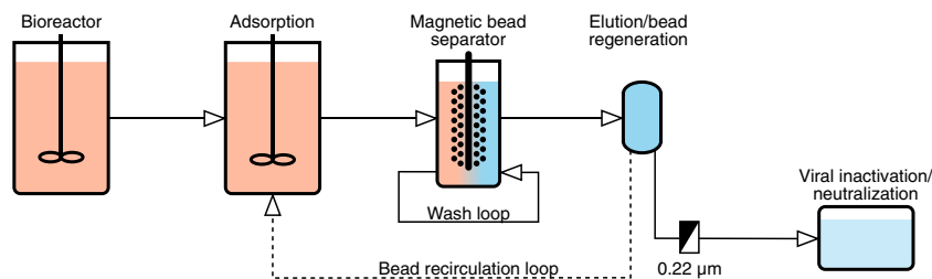
Figure 2. Schematic representation of the pilot-scale magnetic separation system used herein.
