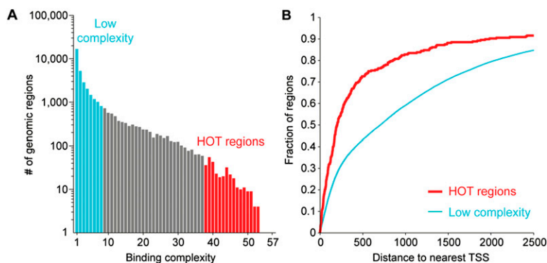
Figure 2. Highly occupied target (HOT) regions. (A) The histogram indicates the number of genomic regions observed for different binding complexities. In blue, thousands of low-complexity regions are bound by eight or fewer factors; in red, 296 HOT regions are bound by 38 or more transcription factors. (B) HOT regions tend to be located close to the transcription start sites (TSSs) of genes. The cumulative distribution plot shows the cumulative fraction of regions (y-axis) that have a maximal distance to the nearest annotated TSS indicated on the x-axis. HOT regions have significantly shorter distances to nearby TSSs than low-complexity regions ( P = 1.7 \times 10^{-23} ; Kolmogorov-Smirnov test). Results shown here are for all annotated genes (WS220); similar results were observed using only protein-coding genes (data not shown).
