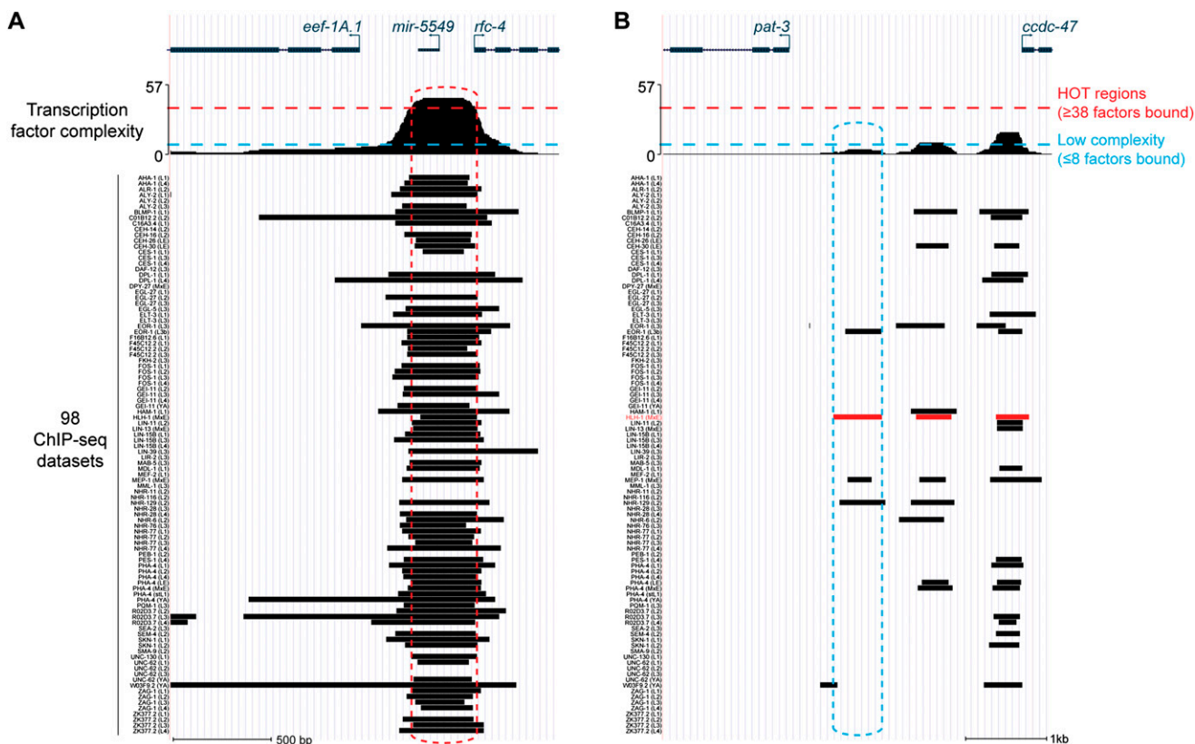
Figure 1. Examples of highly occupied and low-complexity regions of transcription factor binding. Binding of 57 transcription factors in one or more developmental stages (98 ChIP-seq data sets in total) were obtained from the C. elegans modENCODE Consortium and are shown for two examples. Data sets are shown in identical order to Supplemental Table 1. (A) Binding proximal to translation elongation factor 1-alpha homolog eef-1A.1 . An ~450-nt HOT region indicated by the red dashed box is significantly enriched for binding in ChIP-seq analyses of 44 different transcription factors. Transcription factor complexity (the number of factors with ChIP-seq binding sites overlapping that position) is shown at the top. (Below) Regions of significant enrichment ( Q -value \leq 10^{-3} ) observed in each of the 98 ChIP-seq data sets are shown as black boxes. (B) Low-complexity HLH-1 binding region proximal to HLH-1-activated target pat-3 is shown.
