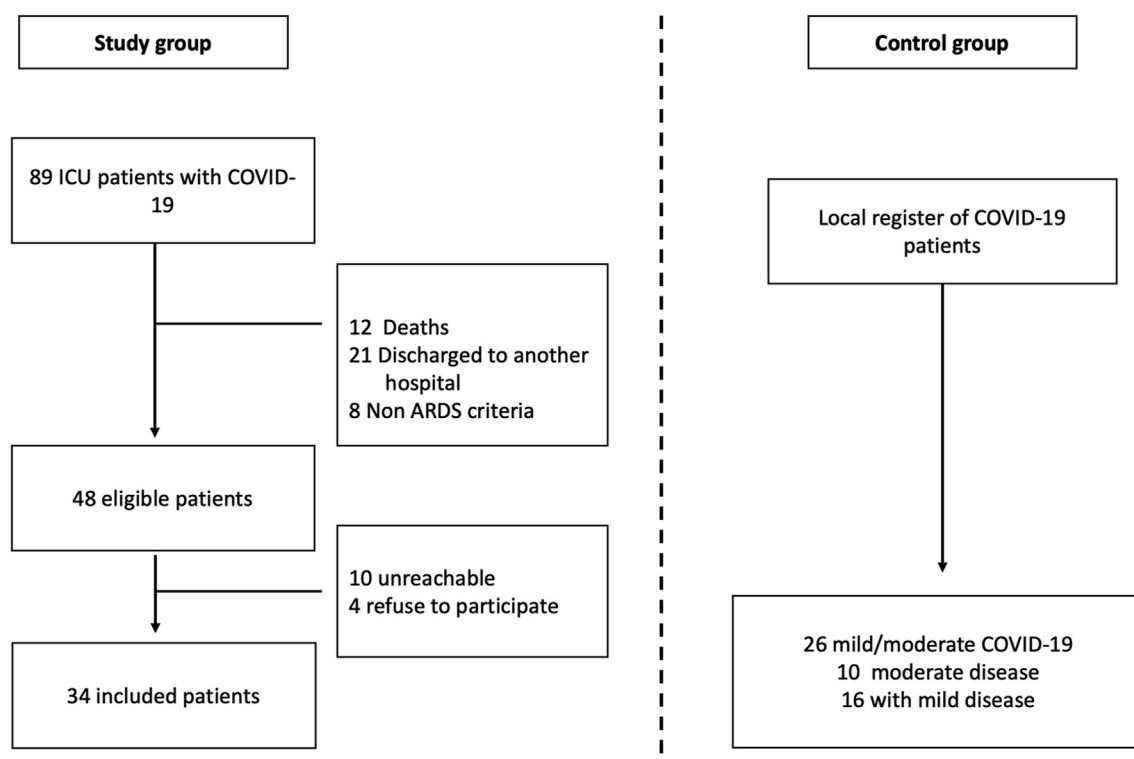
Fig. 1. Study flowchart.
